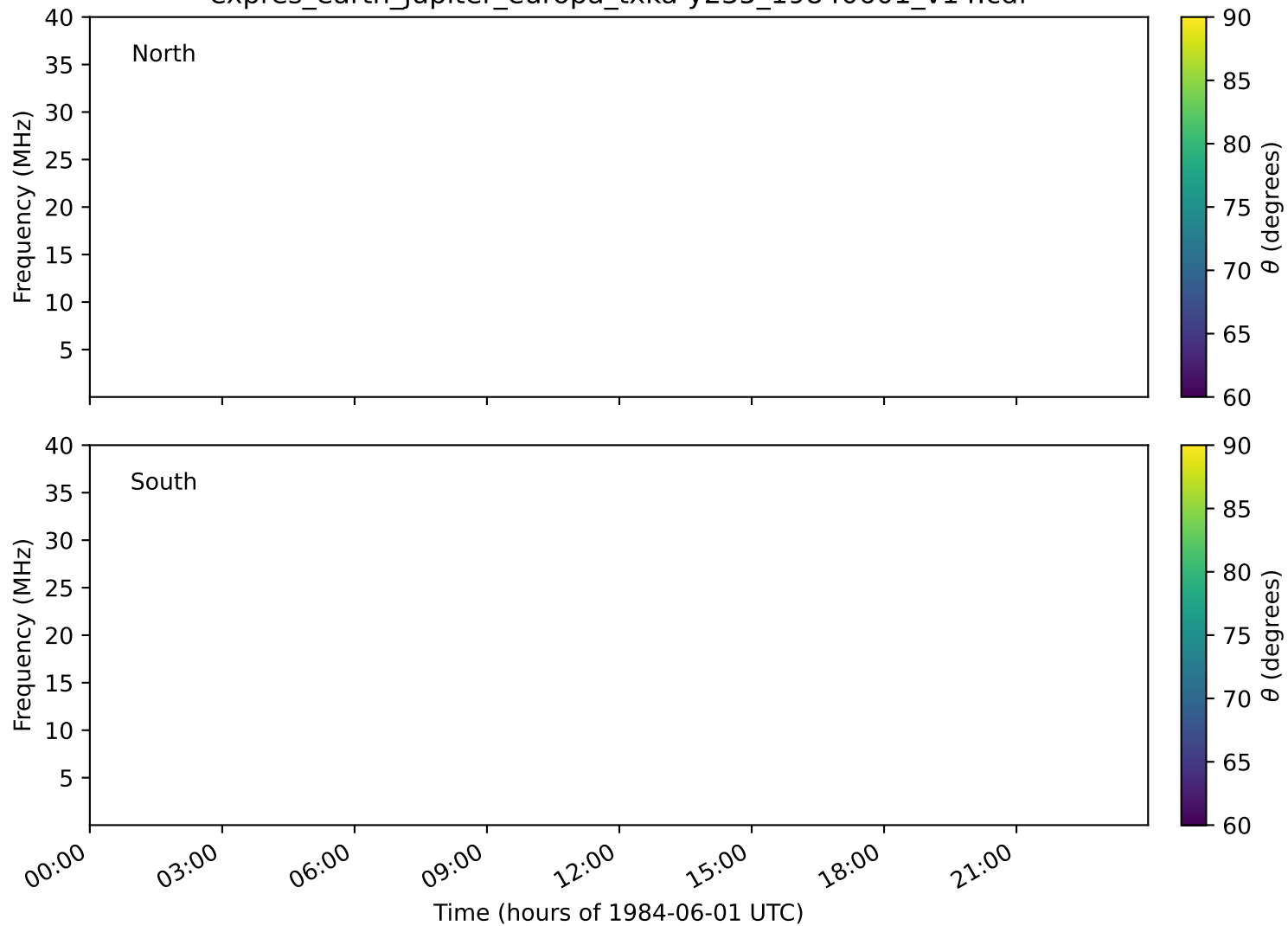
expres_earth_jupiter_europa_txka-y235_19840601_v14.cdf
