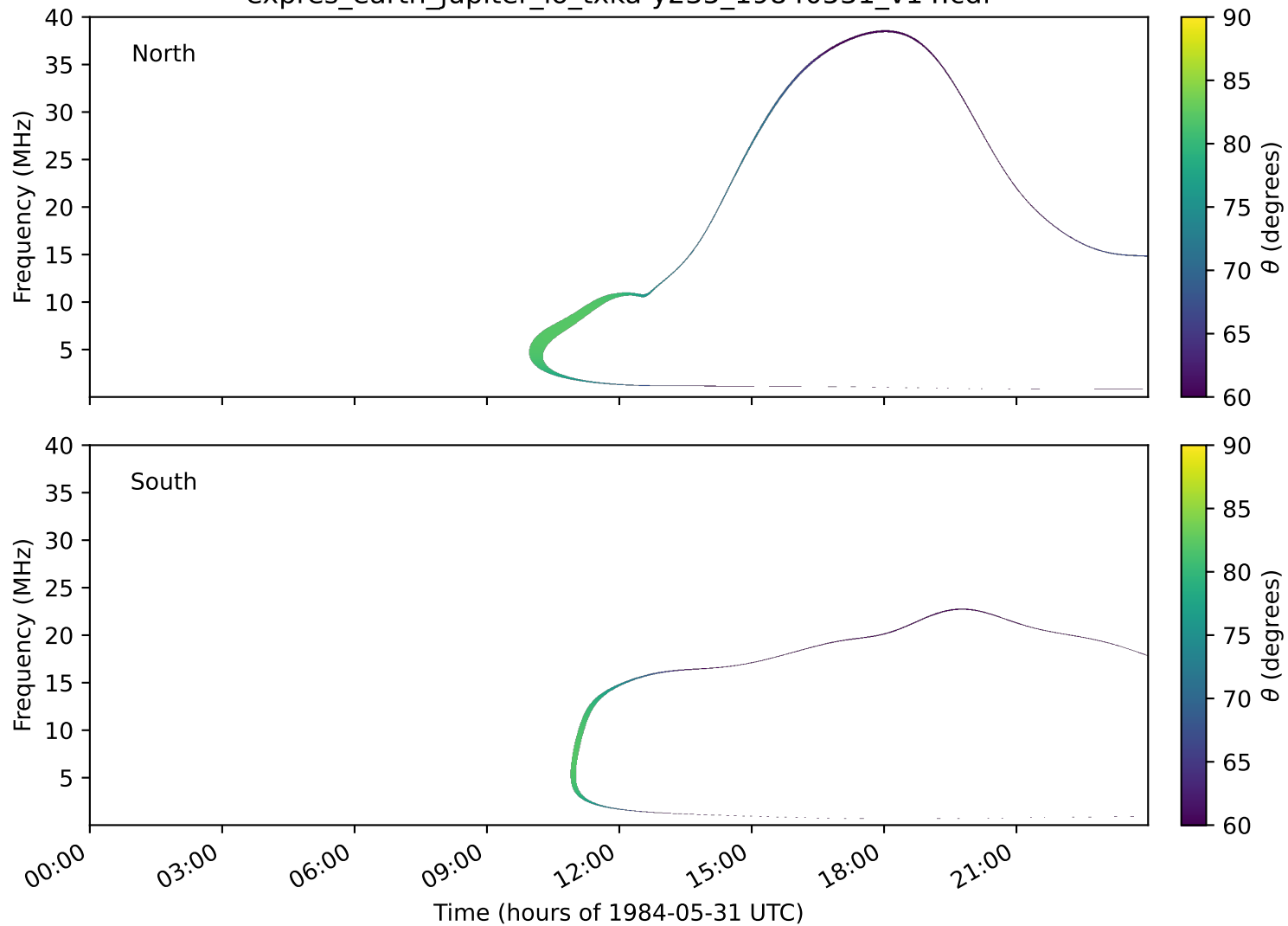
expres_earth_jupiter_io_txka-y235_19840531_v14.cdf
