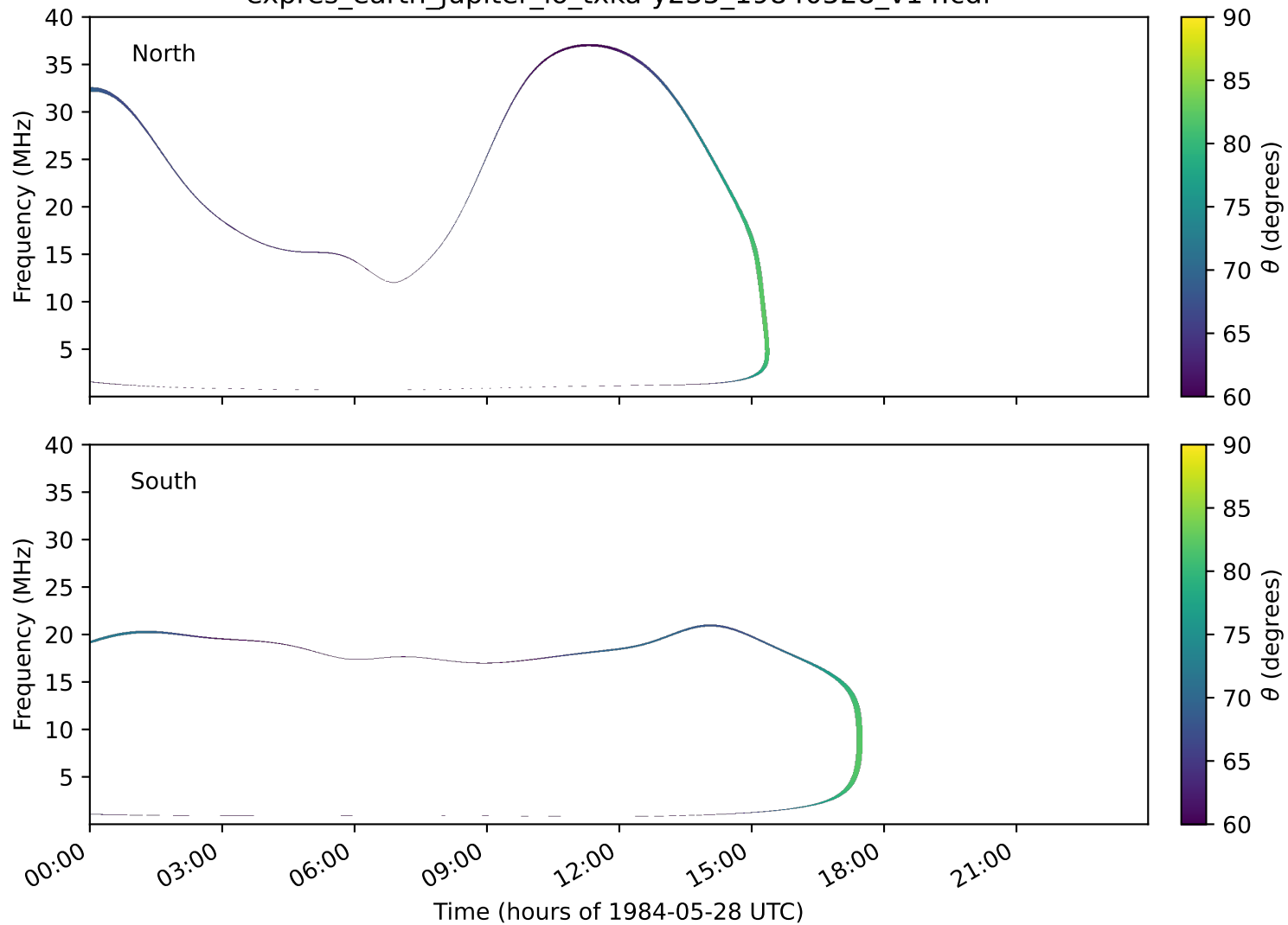
expres_earth_jupiter_io_txka-y235_19840528_v14.cdf
