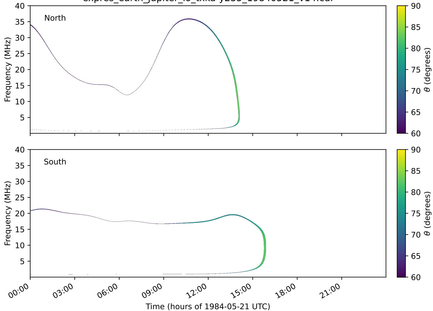
expres_earth_jupiter_io_txka-y235_19840521_v14.cdf
