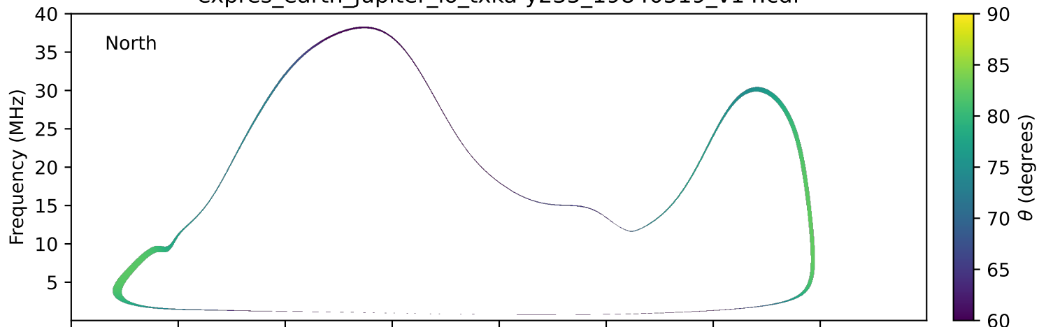
expres_earth_jupiter_io_txka-y235_19840519_v14.cdf
