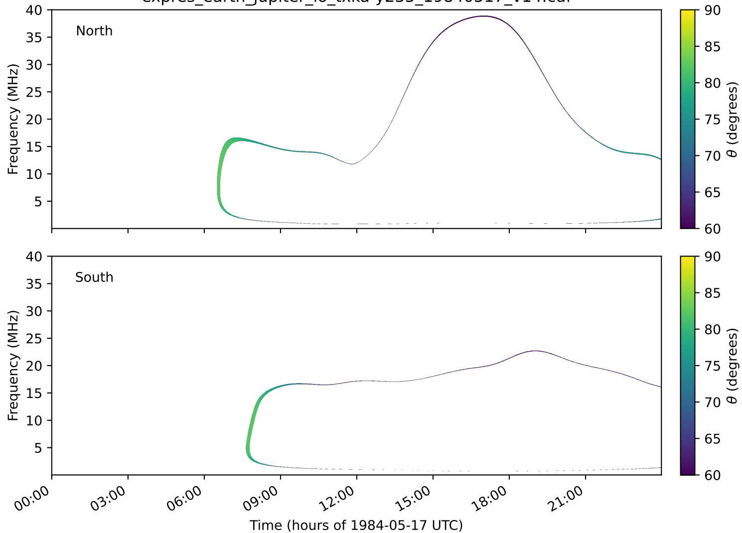
expres_earth_jupiter_io_txka-y235_19840517_v14.cdf
