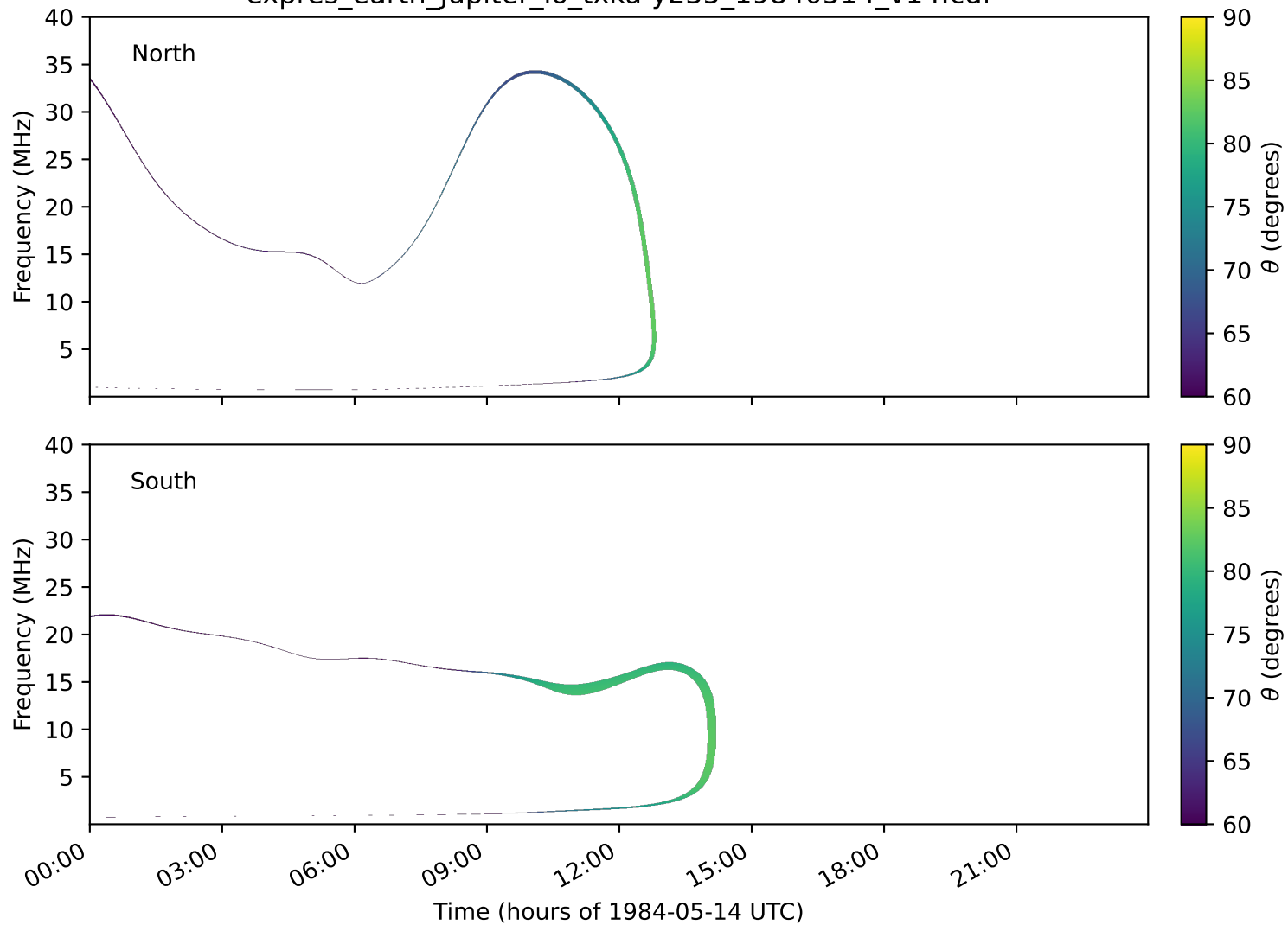
expres_earth_jupiter_io_txka-y235_19840514_v14.cdf
