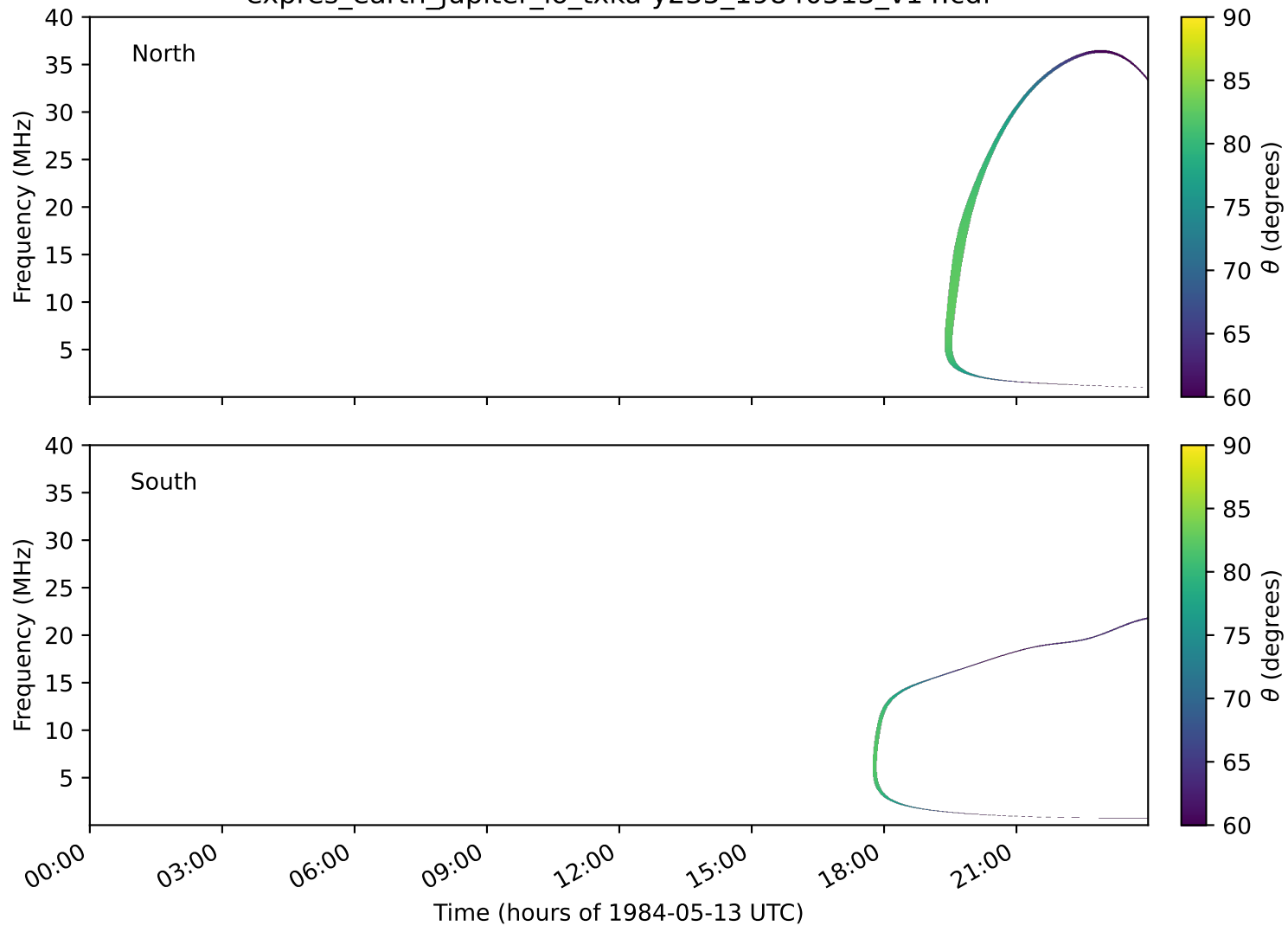
expres_earth_jupiter_io_txka-y235_19840513_v14.cdf
