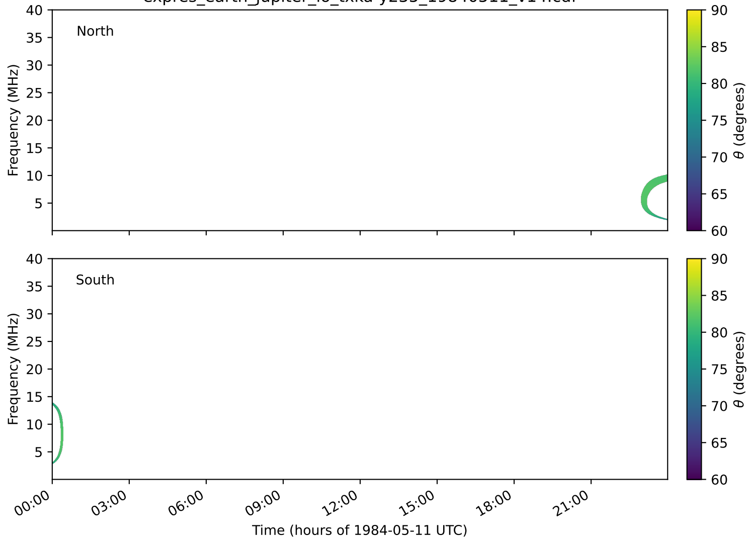
expres_earth_jupiter_io_txka-y235_19840511_v14.cdf
