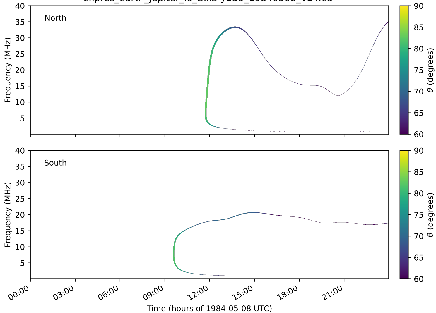
expres_earth_jupiter_io_txka-y235_19840508_v14.cdf
