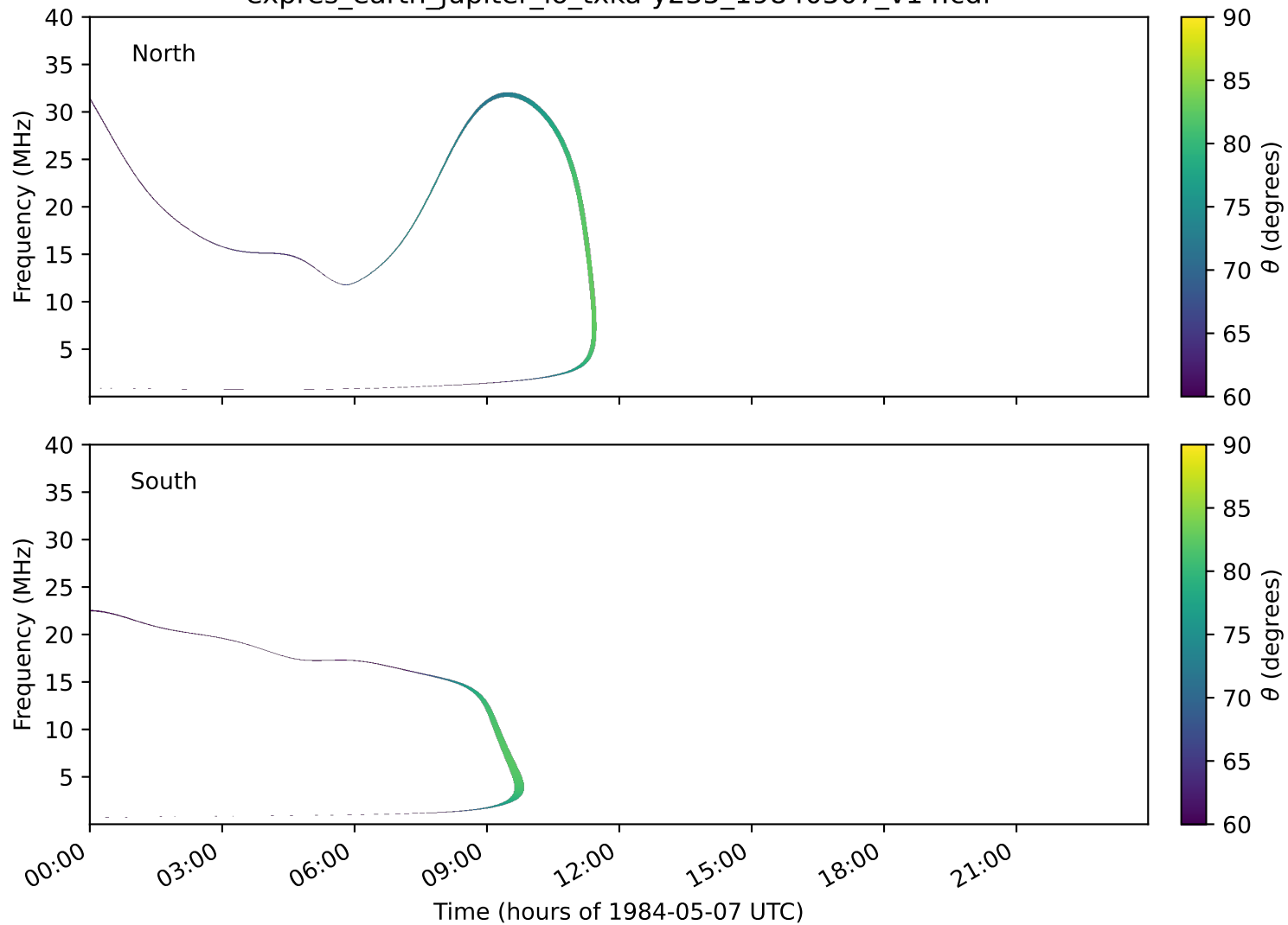
expres_earth_jupiter_io_txka-y235_19840507_v14.cdf
