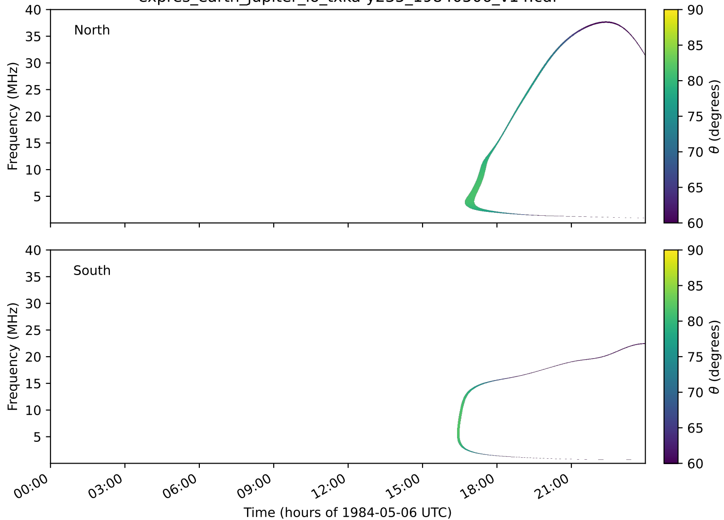
expres_earth_jupiter_io_txka-y235_19840506_v14.cdf
