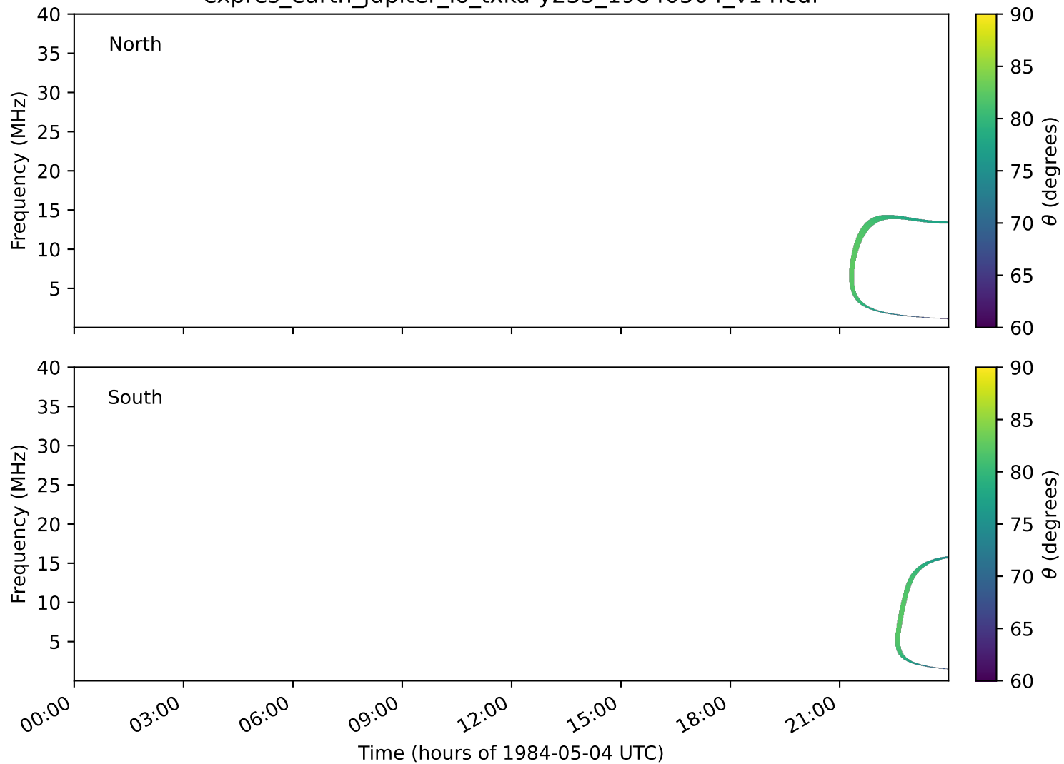
expres_earth_jupiter_io_txka-y235_19840504_v14.cdf
