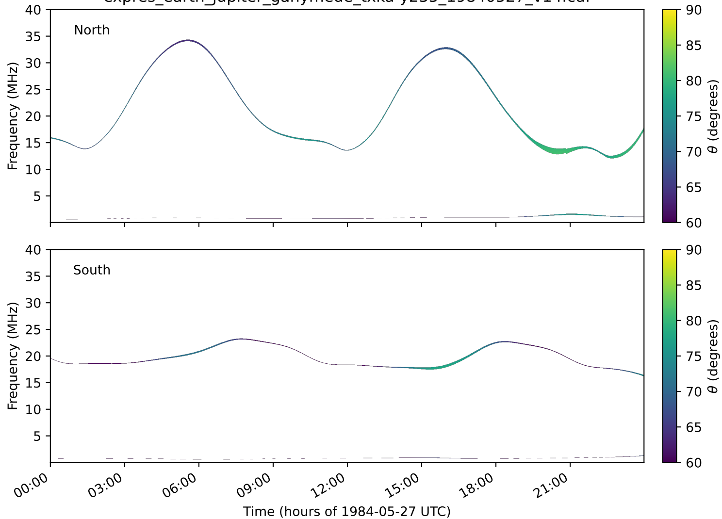
expres_earth_jupiter_ganymede_txka-y235_19840527_v14.cdf
