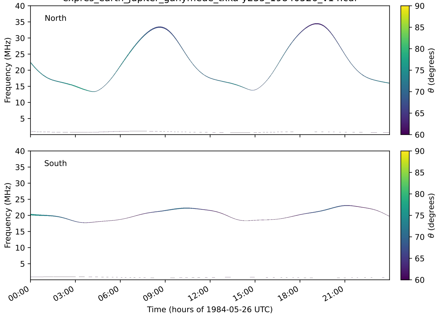
expres_earth_jupiter_ganymede_txka-y235_19840526_v14.cdf
