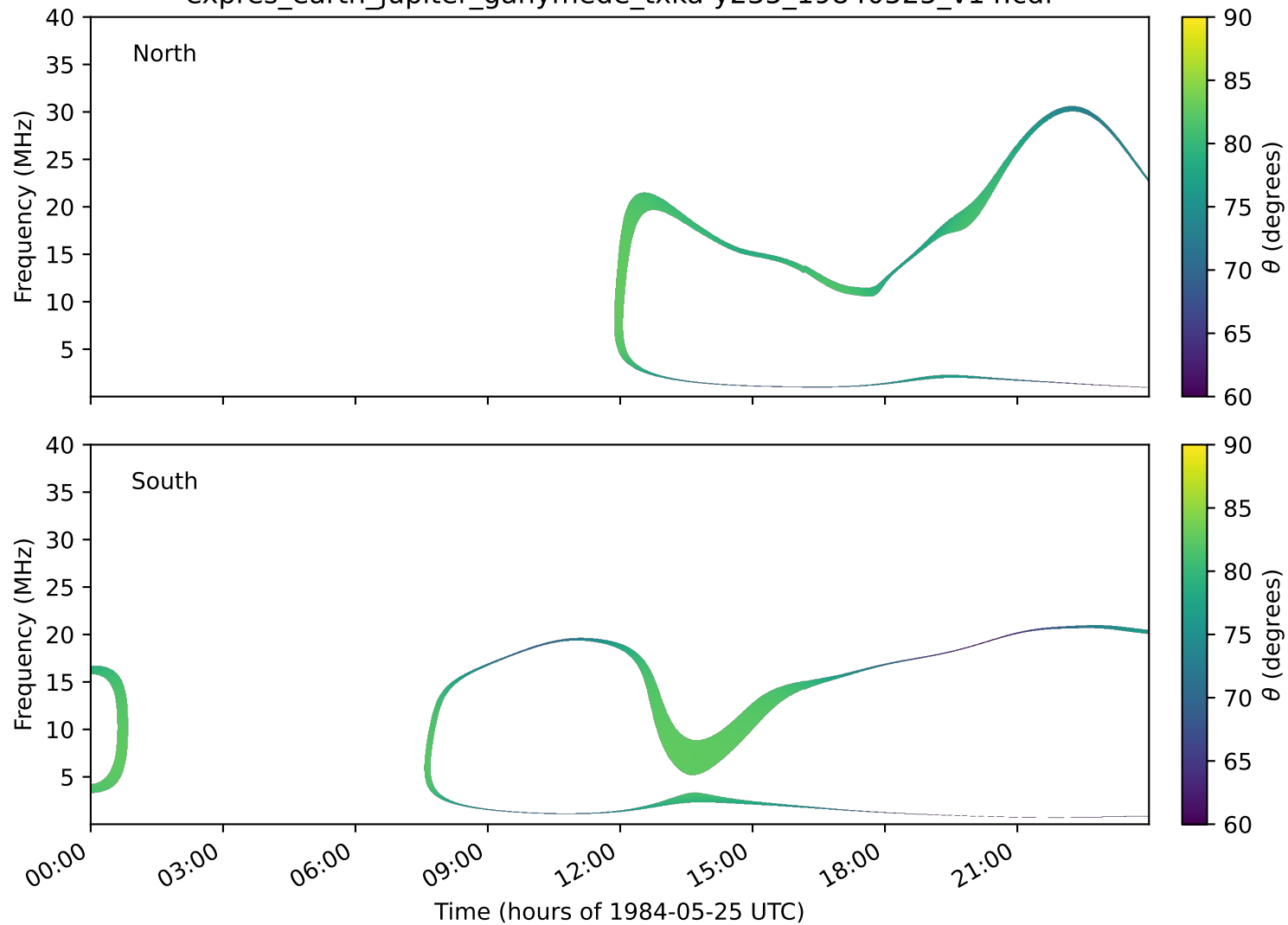
expres_earth_jupiter_ganymede_txka-y235_19840525_v14.cdf
