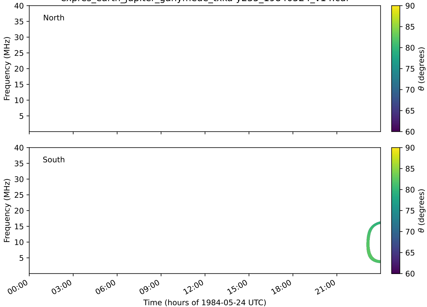
expres_earth_jupiter_ganymede_txka-y235_19840524_v14.cdf
