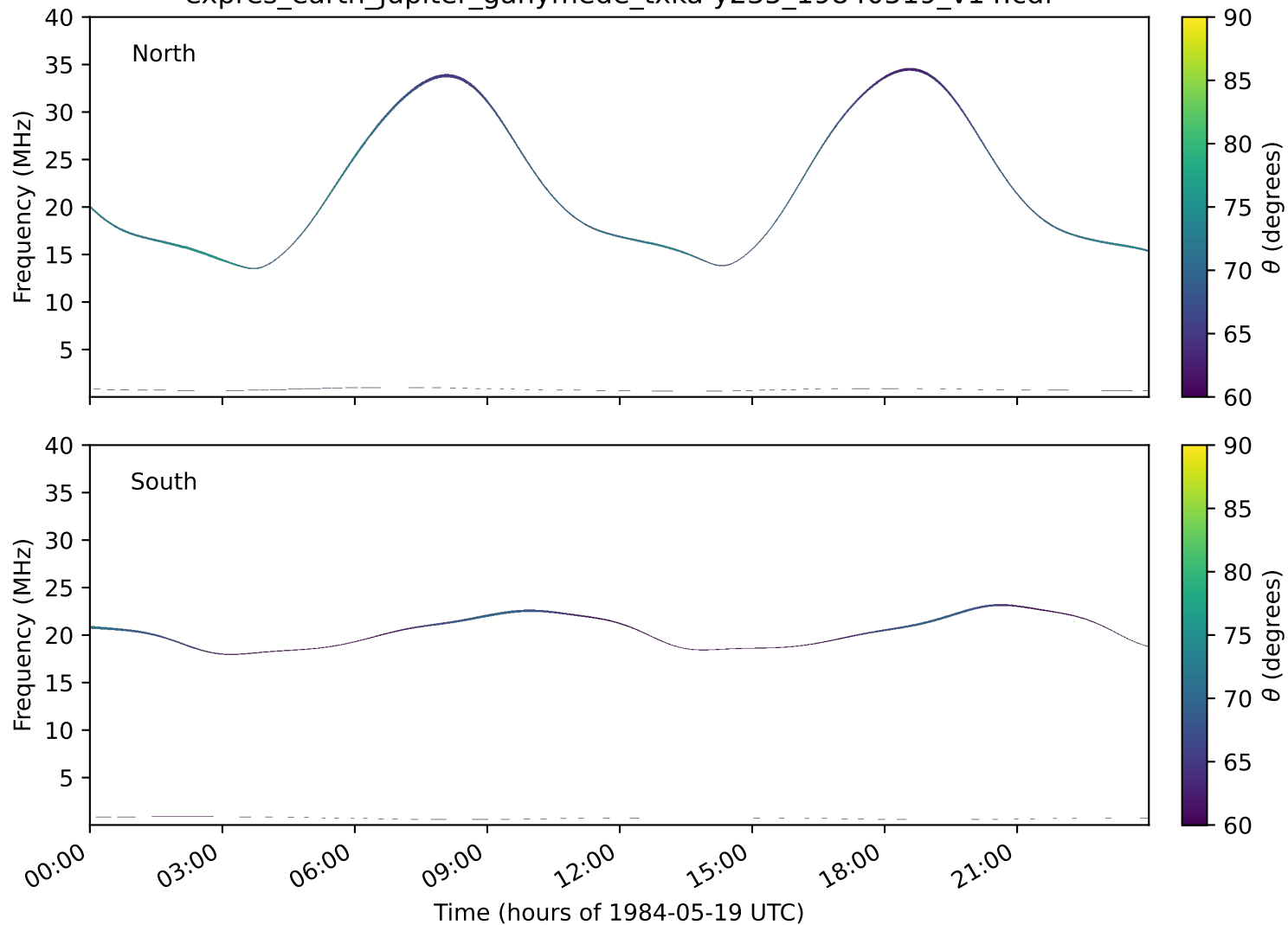
expres_earth_jupiter_ganymede_txka-y235_19840519_v14.cdf
