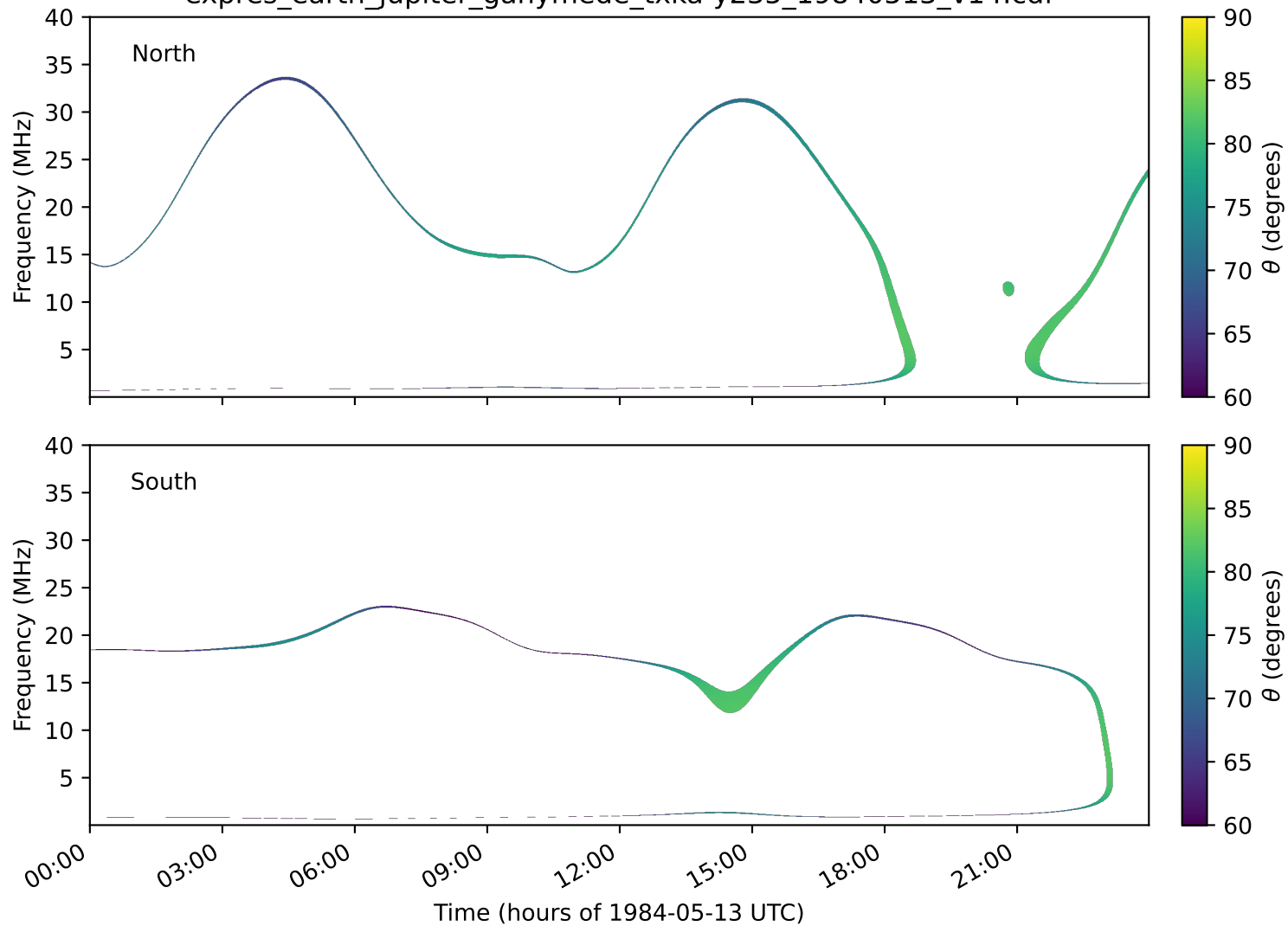
expres_earth_jupiter_ganymede_txka-y235_19840513_v14.cdf
