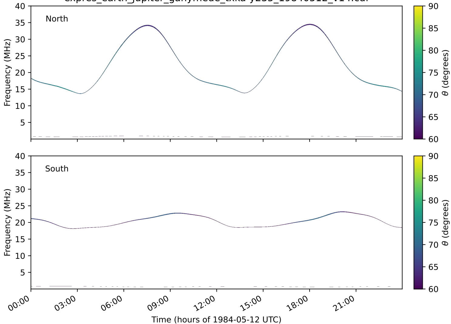
expres_earth_jupiter_ganymede_txka-y235_19840512_v14.cdf
