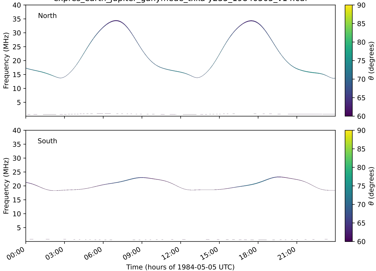
expres_earth_jupiter_ganymede_txka-y235_19840505_v14.cdf
