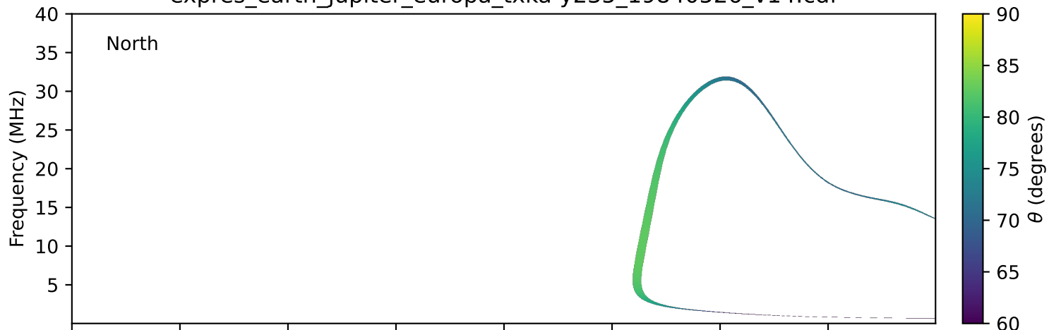
expres_earth_jupiter_europa_txka-y235_19840526_v14.cdf
