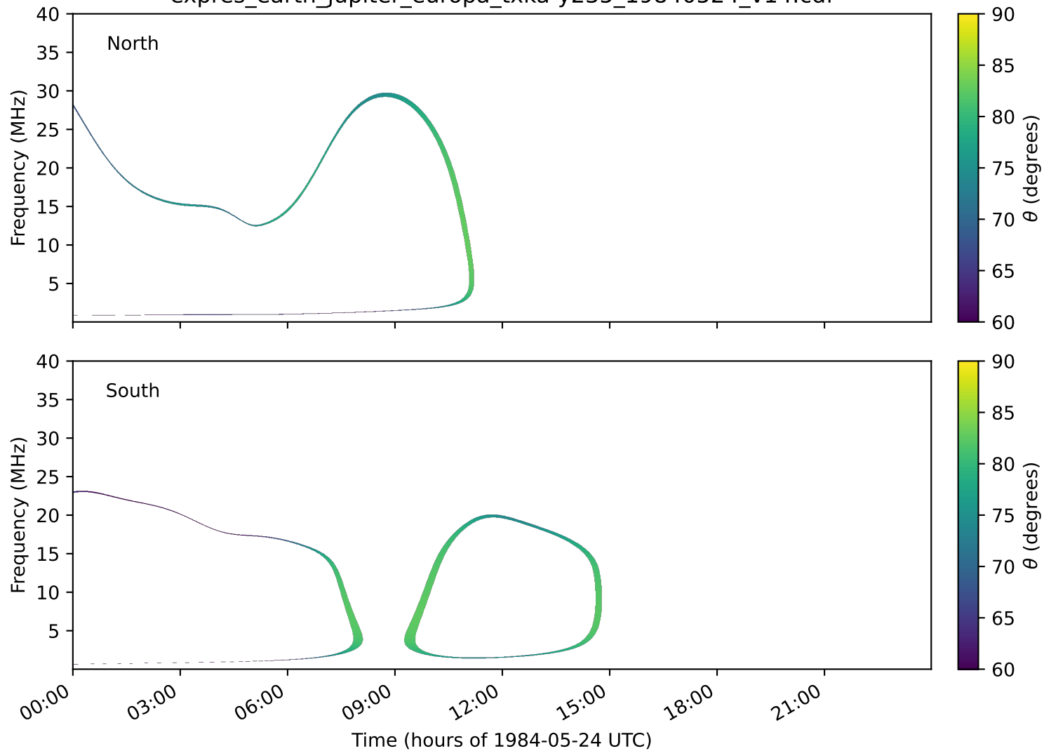
expres_earth_jupiter_europa_txka-y235_19840524_v14.cdf
