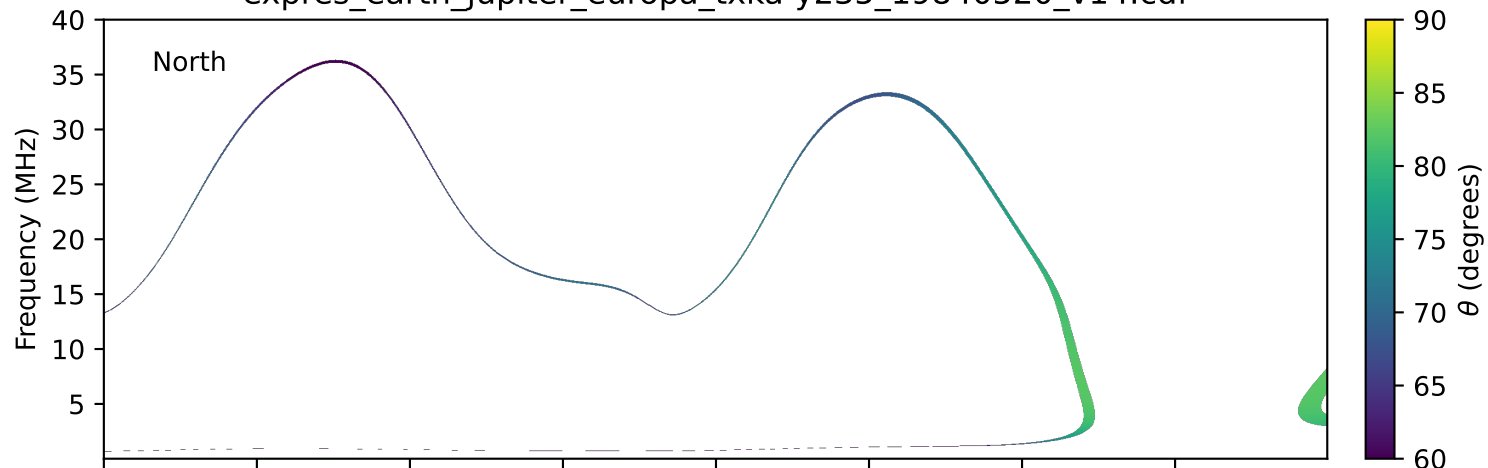
expres_earth_jupiter_europa_txka-y235_19840520_v14.cdf
