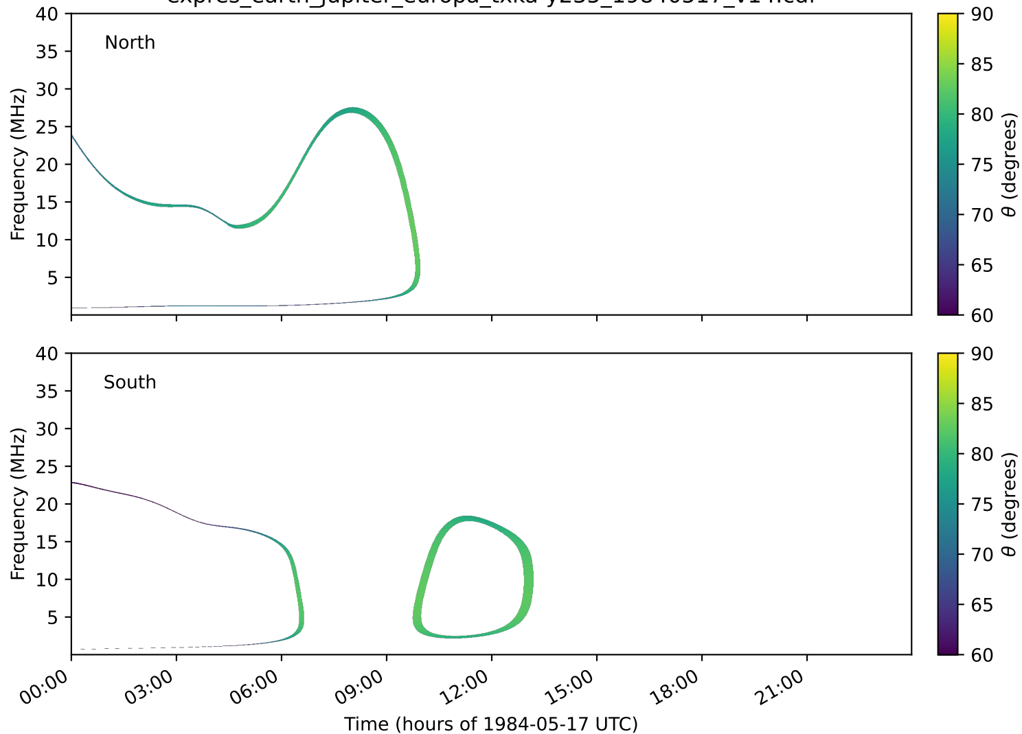
expres_earth_jupiter_europa_txka-y235_19840517_v14.cdf
