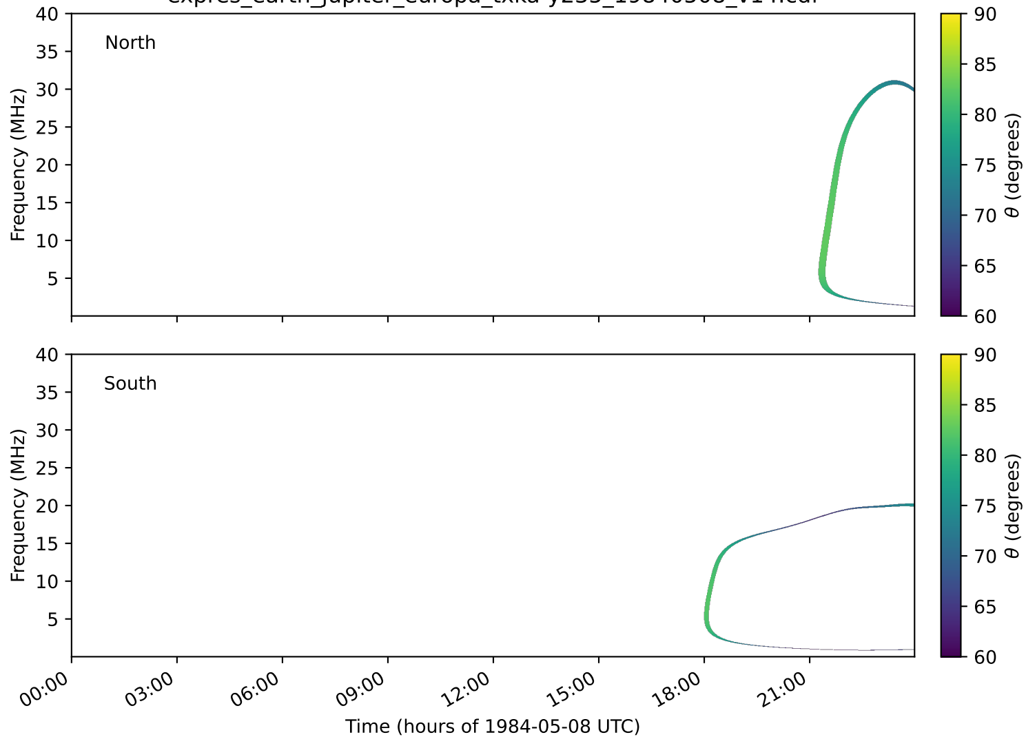
expres_earth_jupiter_europa_txka-y235_19840508_v14.cdf
