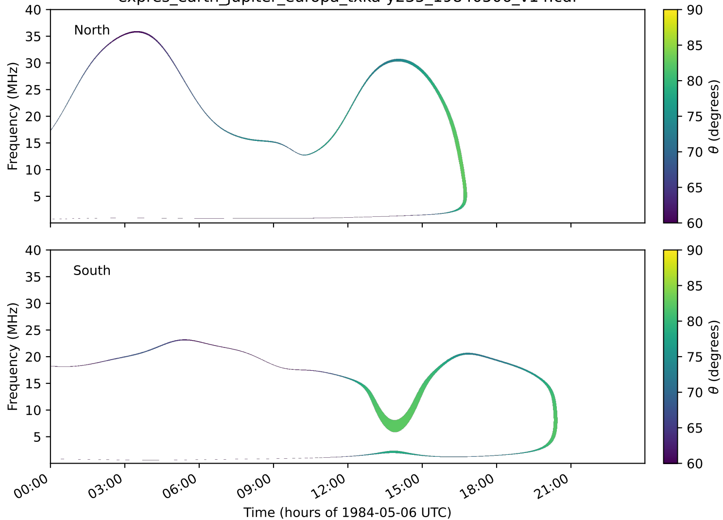
expres_earth_jupiter_europa_txka-y235_19840506_v14.cdf
