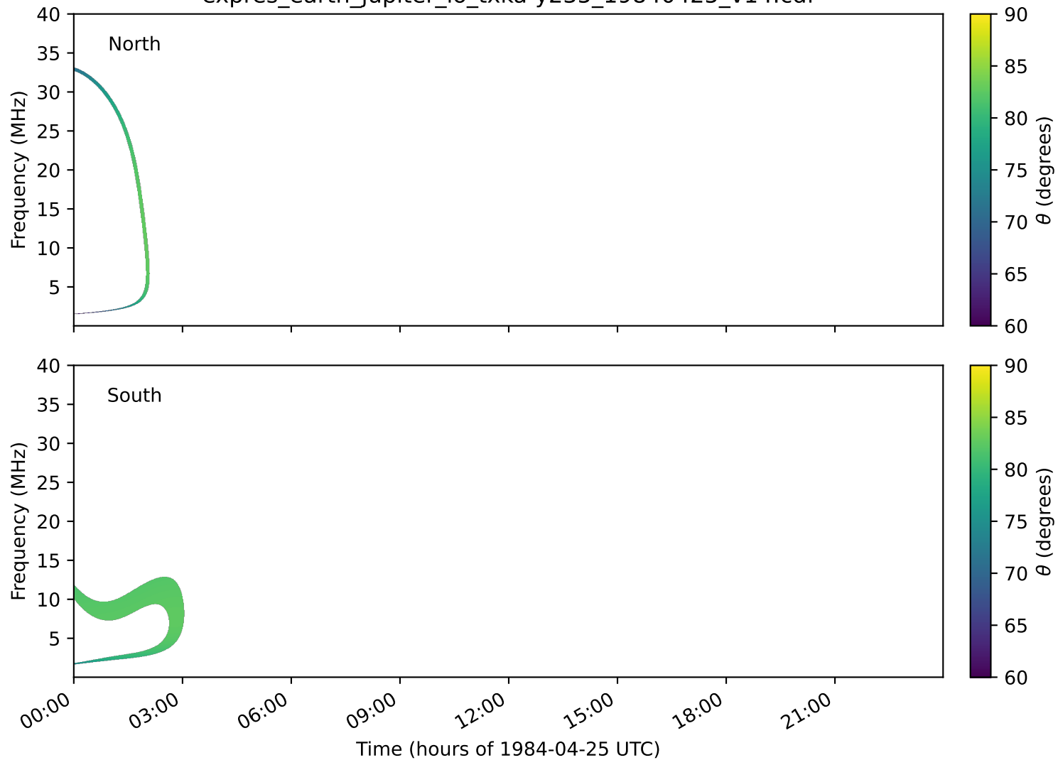
expres_earth_jupiter_io_txka-y235_19840425_v14.cdf
