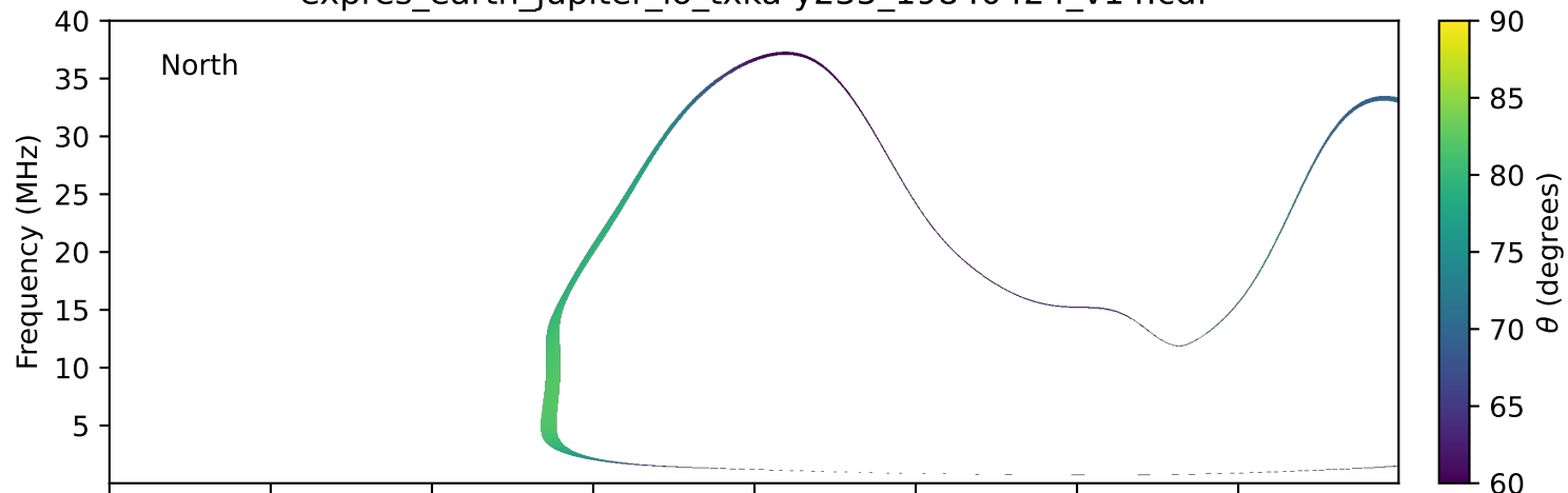
expres_earth_jupiter_io_txka-y235_19840424_v14.cdf
