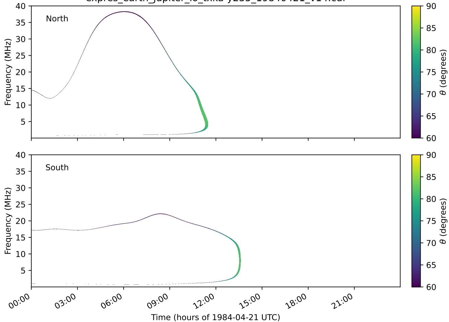
expres_earth_jupiter_io_txka-y235_19840421_v14.cdf
