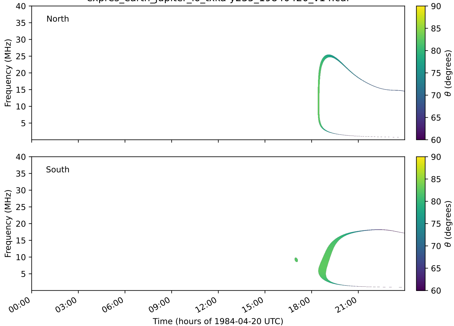
expres_earth_jupiter_io_txka-y235_19840420_v14.cdf
