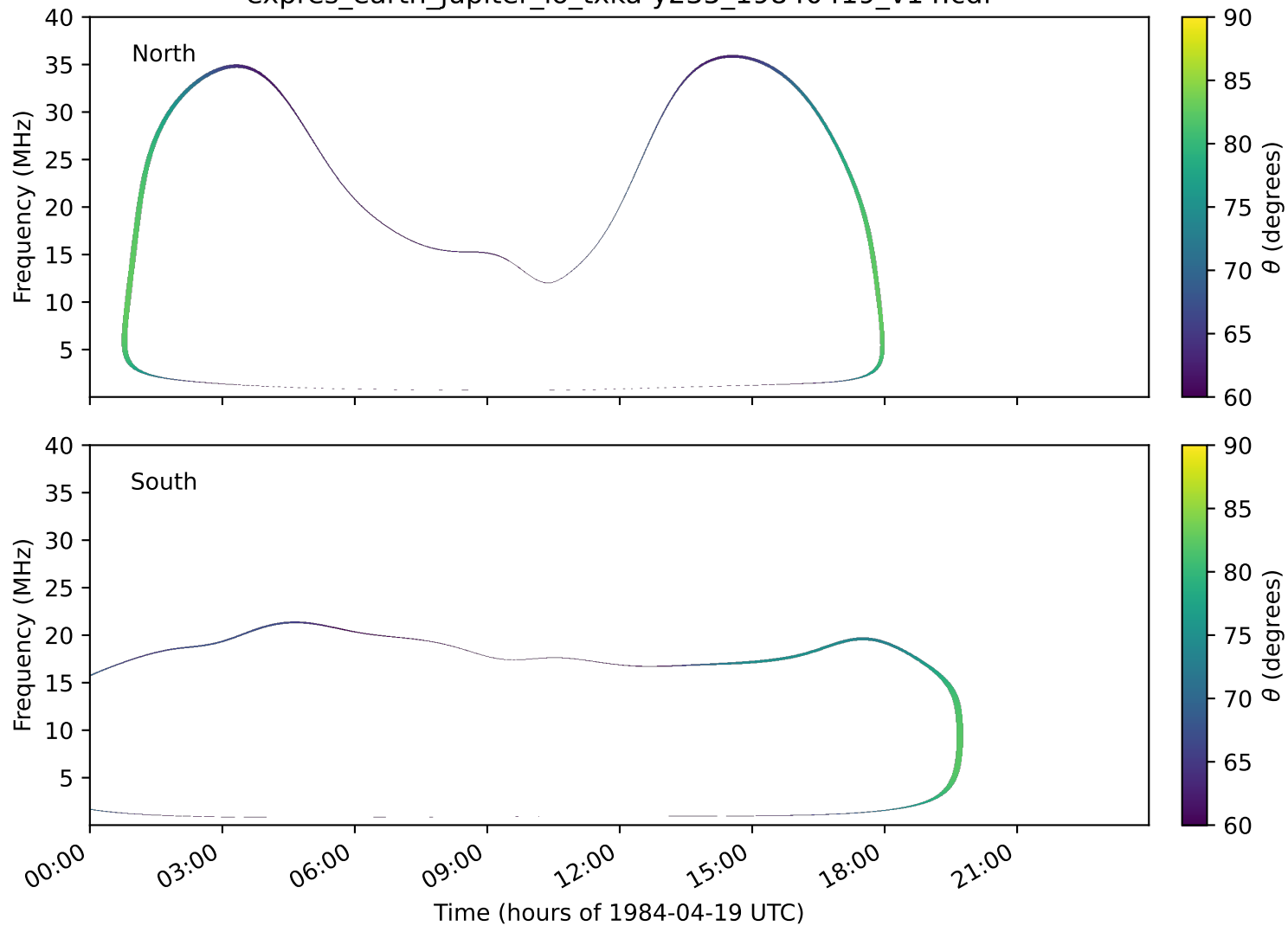
expres_earth_jupiter_io_txka-y235_19840419_v14.cdf
