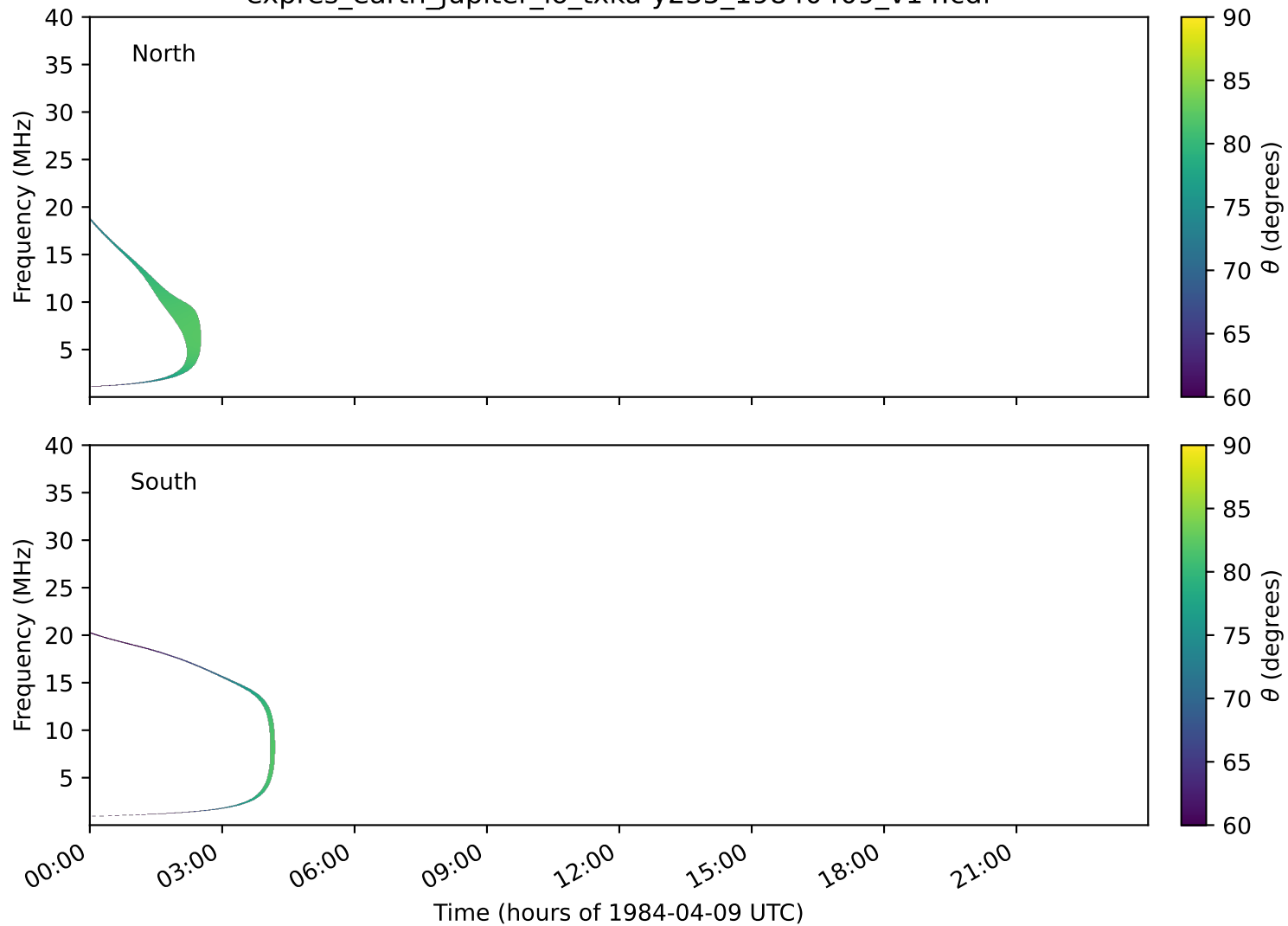
expres_earth_jupiter_io_txka-y235_19840409_v14.cdf
