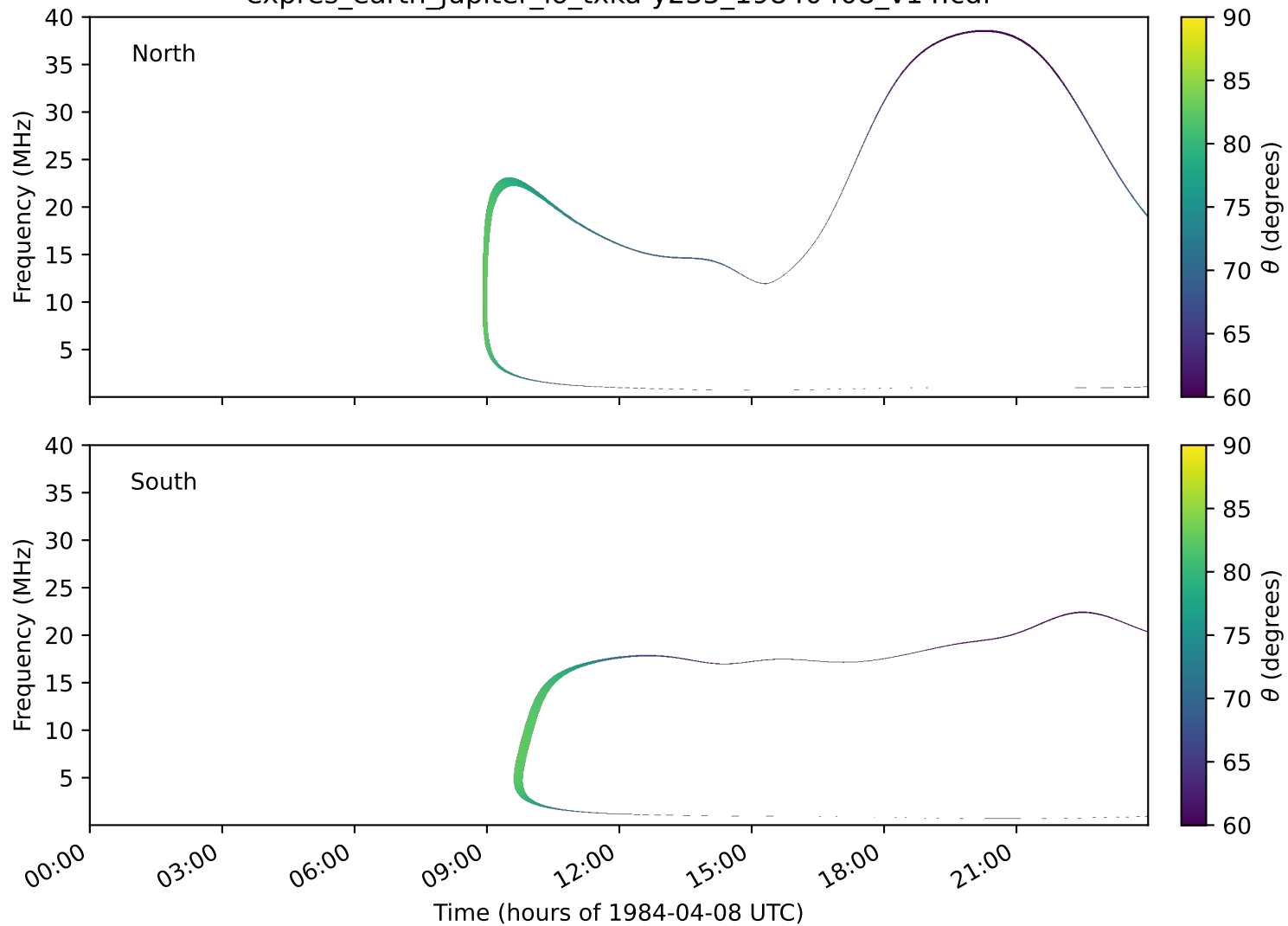
expres_earth_jupiter_io_txka-y235_19840408_v14.cdf
