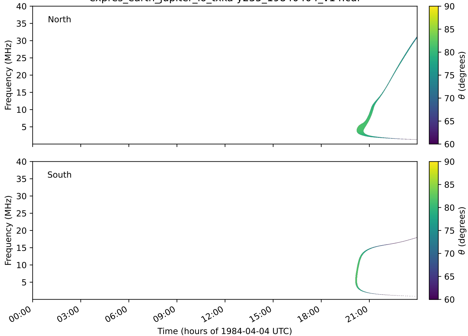
expres_earth_jupiter_io_txka-y235_19840404_v14.cdf
