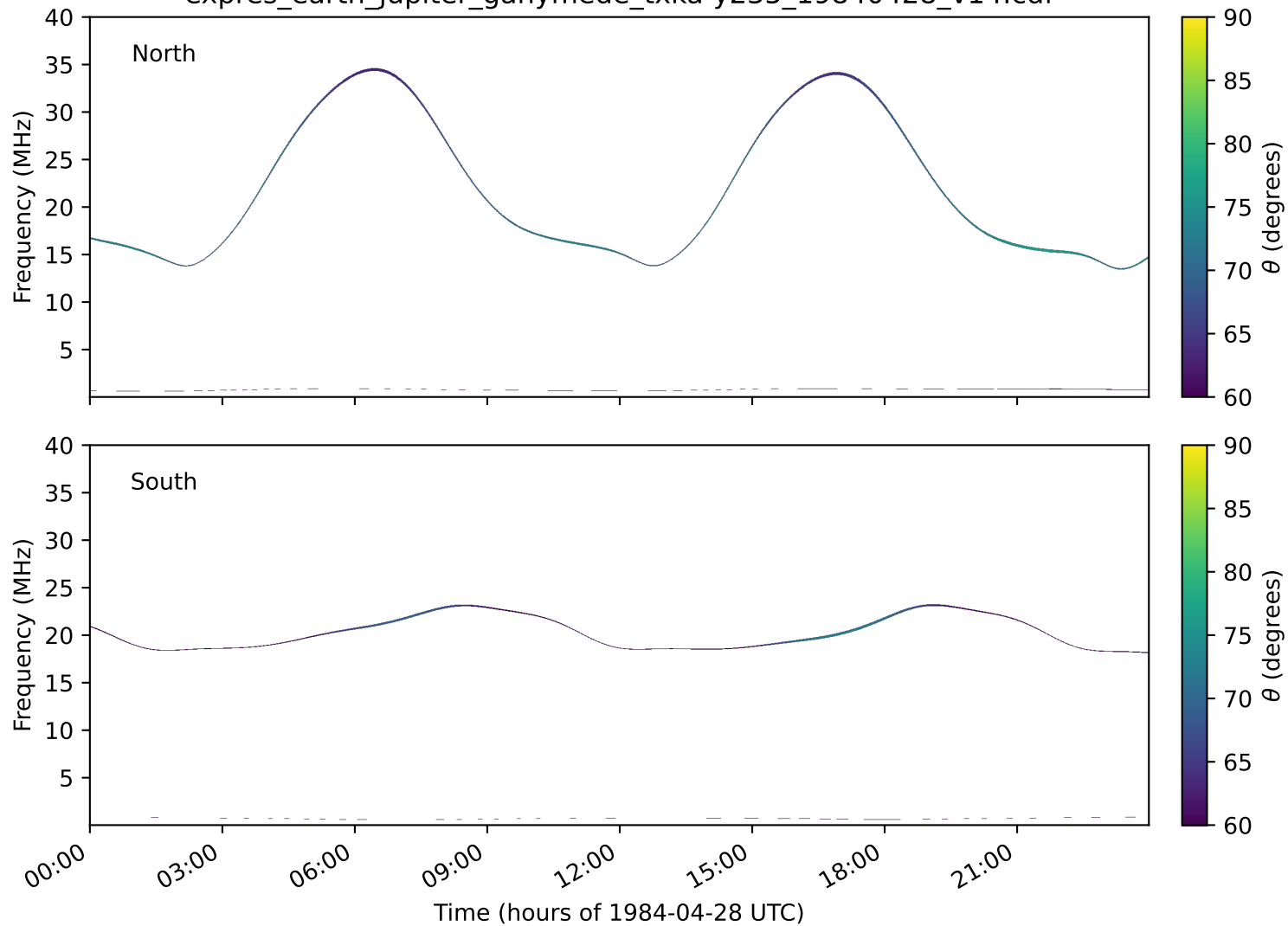
expres_earth_jupiter_ganymede_txka-y235_19840428_v14.cdf
