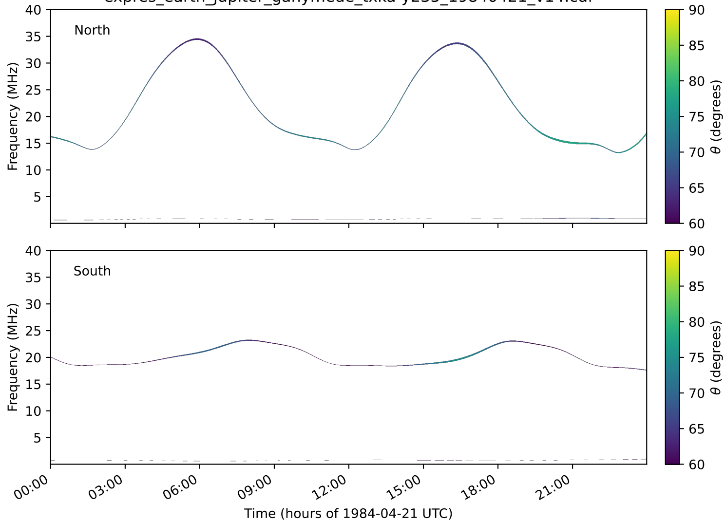
expres_earth_jupiter_ganymede_txka-y235_19840421_v14.cdf
