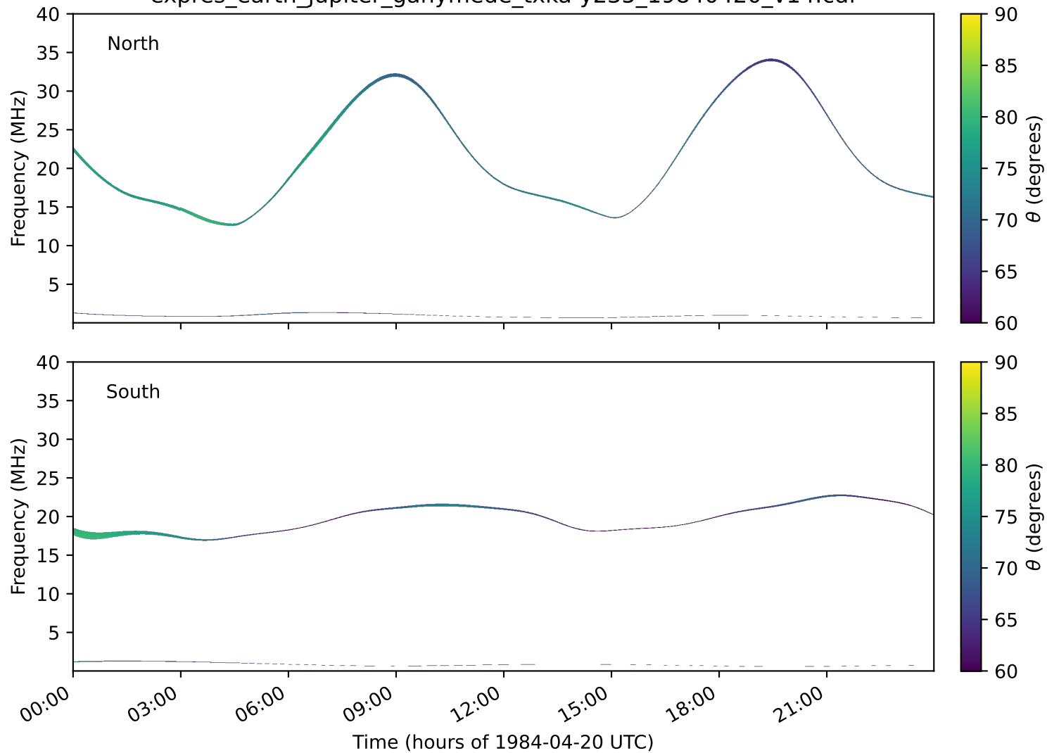
expres_earth_jupiter_ganymede_txka-y235_19840420_v14.cdf
