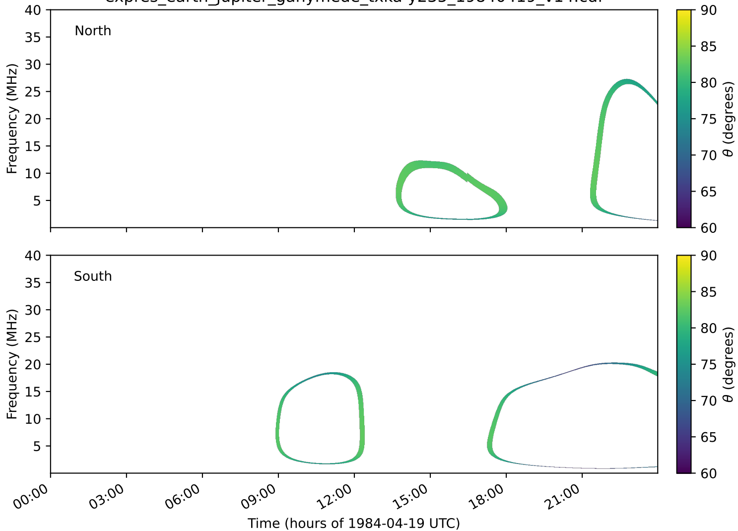
expres_earth_jupiter_ganymede_txka-y235_19840419_v14.cdf
