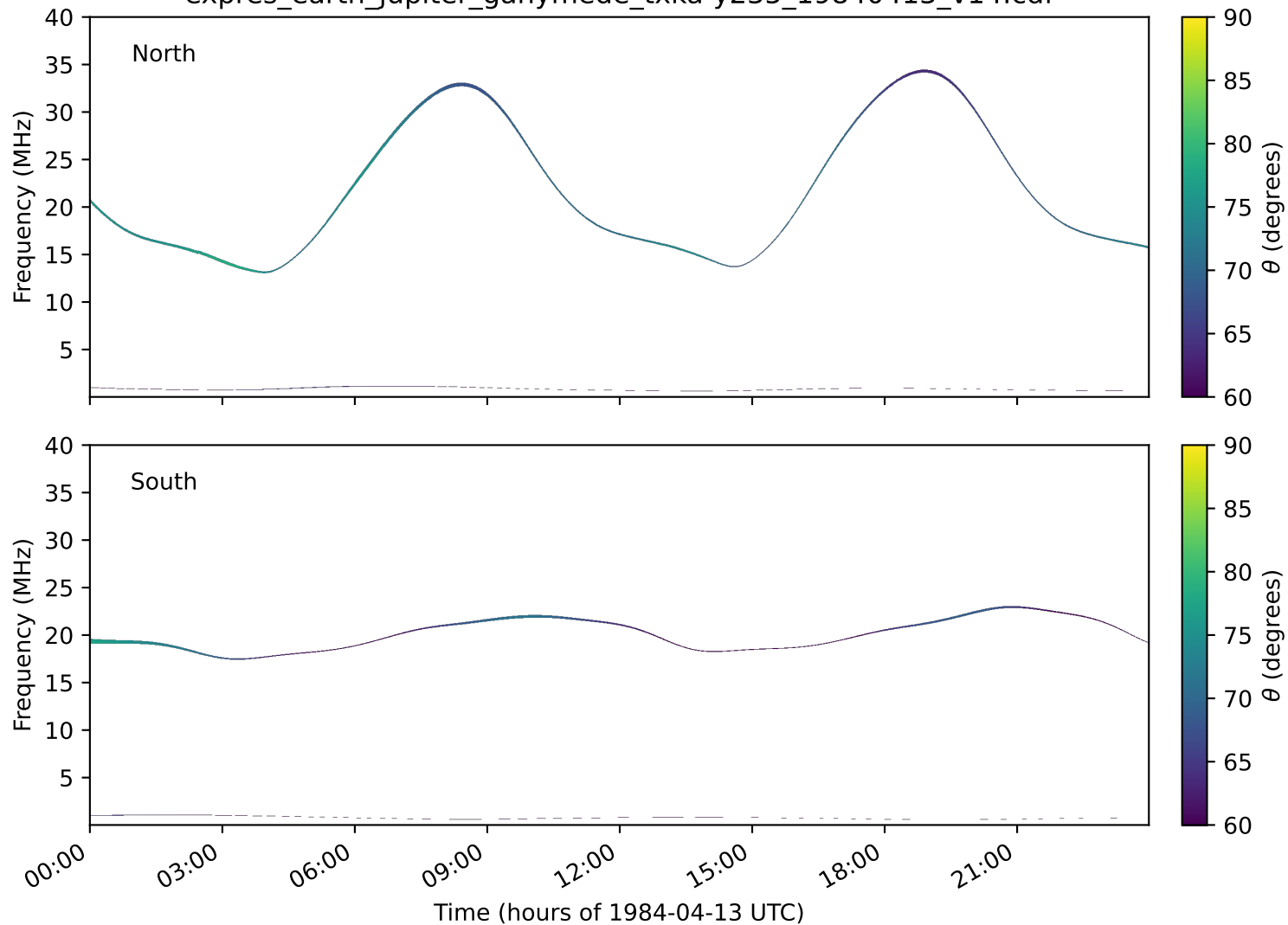
expres_earth_jupiter_ganymede_txka-y235_19840413_v14.cdf
