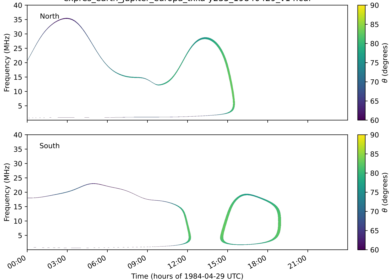
expres_earth_jupiter_europa_txka-y235_19840429_v14.cdf
