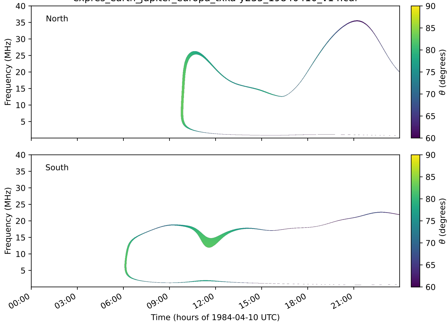
expres_earth_jupiter_europa_txka-y235_19840410_v14.cdf
