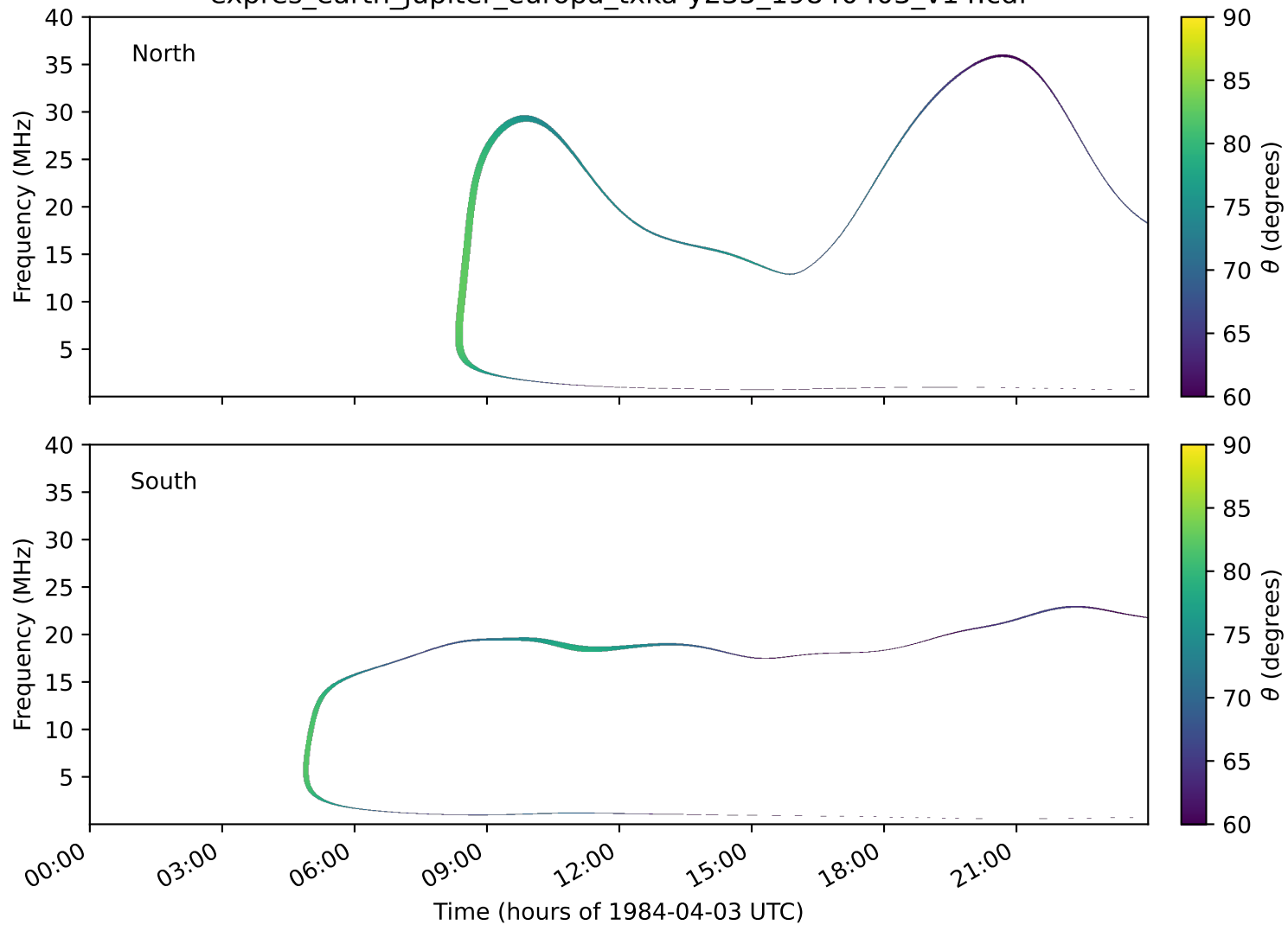
expres_earth_jupiter_europa_txka-y235_19840403_v14.cdf
