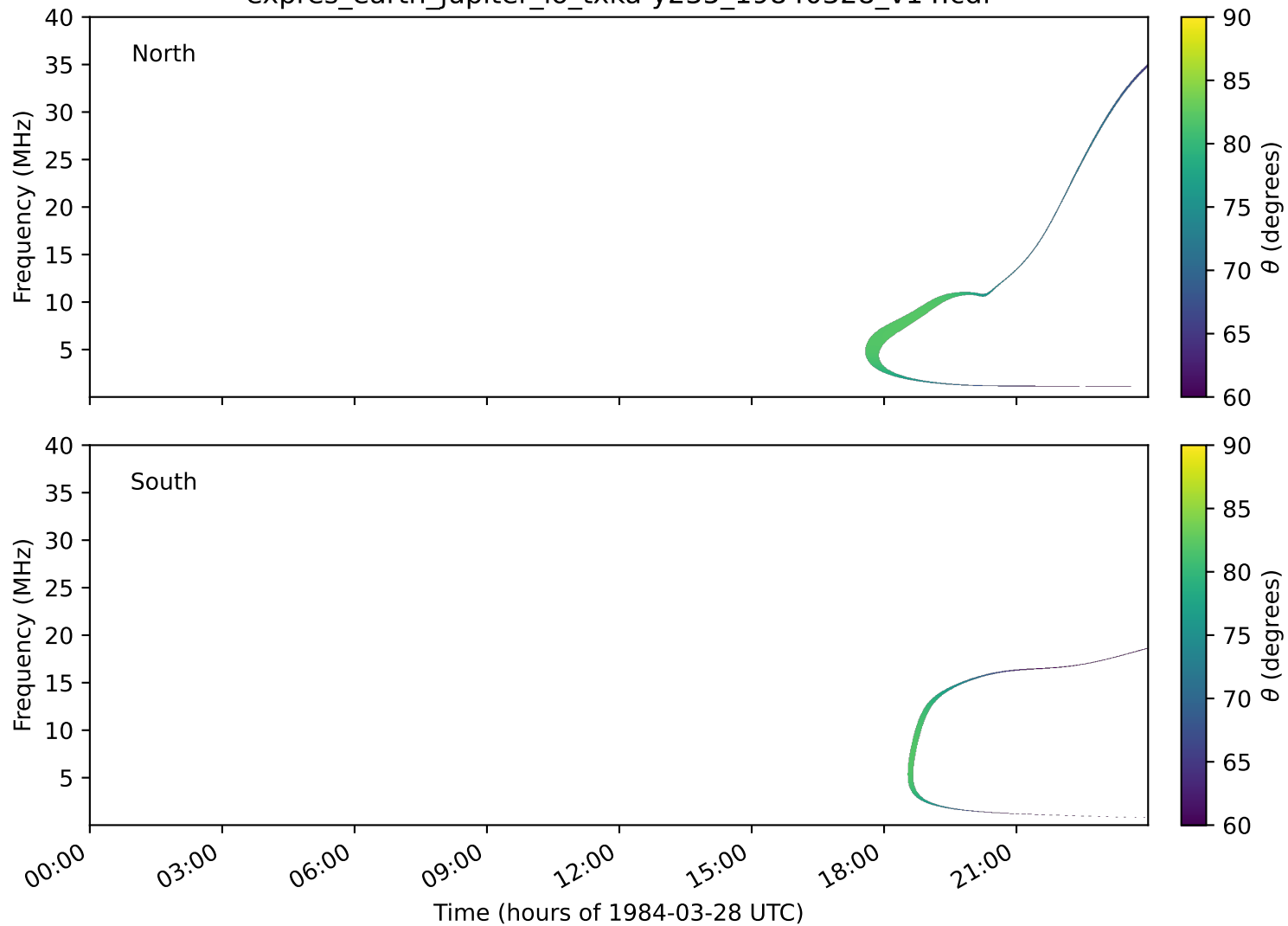
expres_earth_jupiter_io_txka-y235_19840328_v14.cdf
