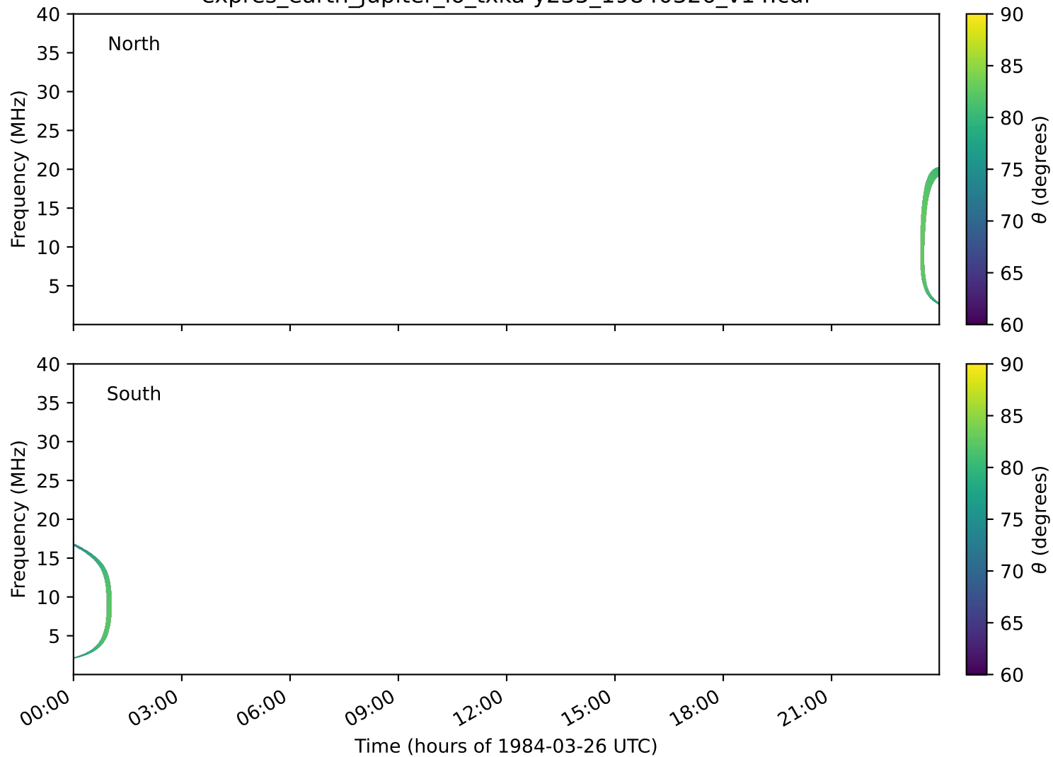
expres_earth_jupiter_io_txka-y235_19840326_v14.cdf
