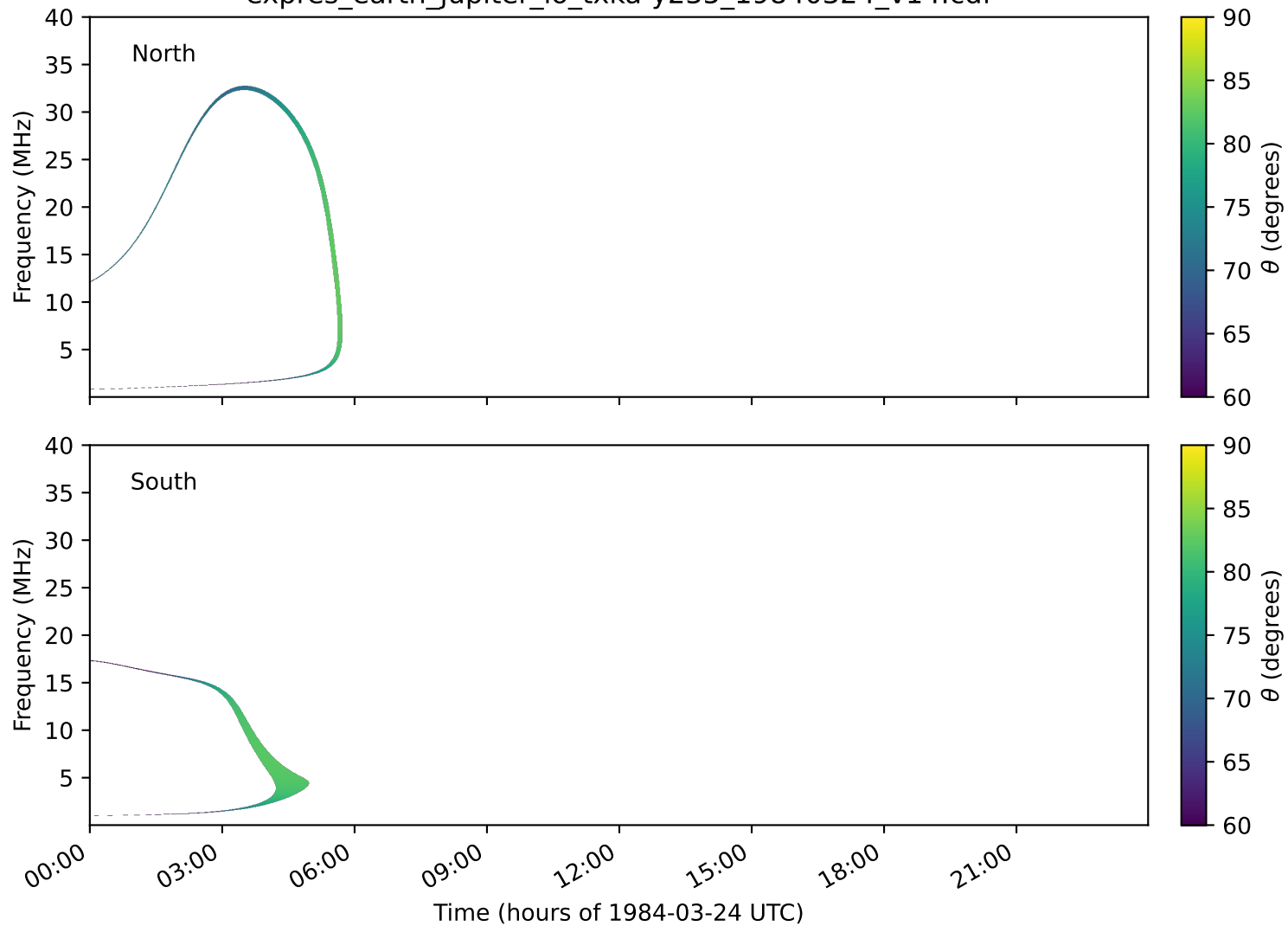
expres_earth_jupiter_io_txka-y235_19840324_v14.cdf
