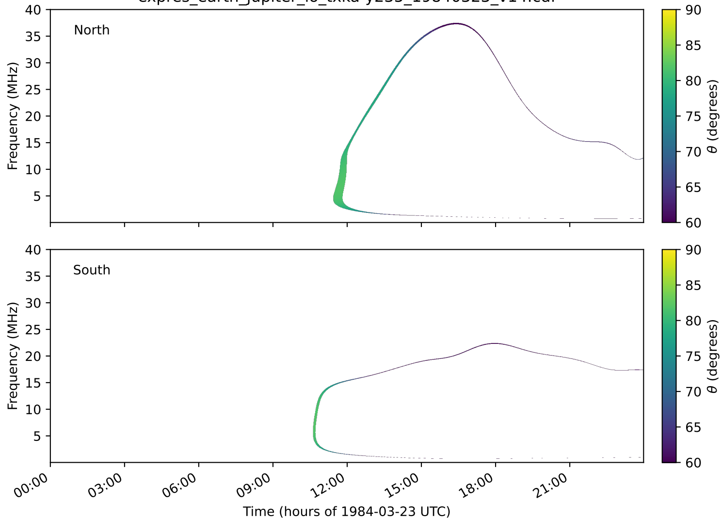
expres_earth_jupiter_io_txka-y235_19840323_v14.cdf
