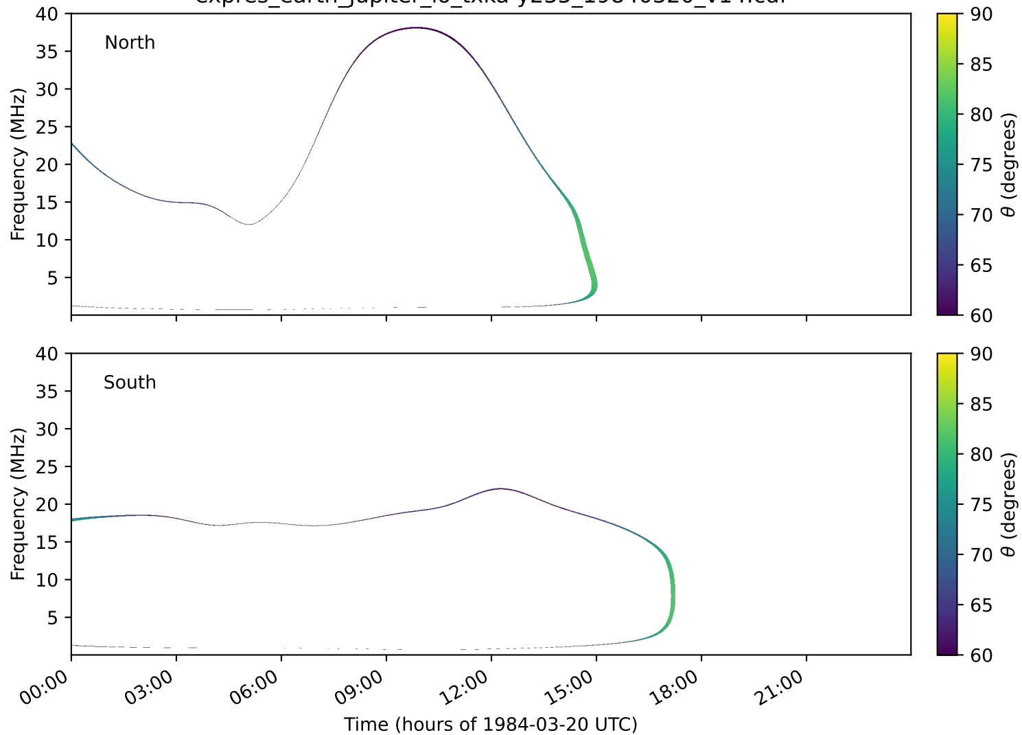
expres_earth_jupiter_io_txka-y235_19840320_v14.cdf
