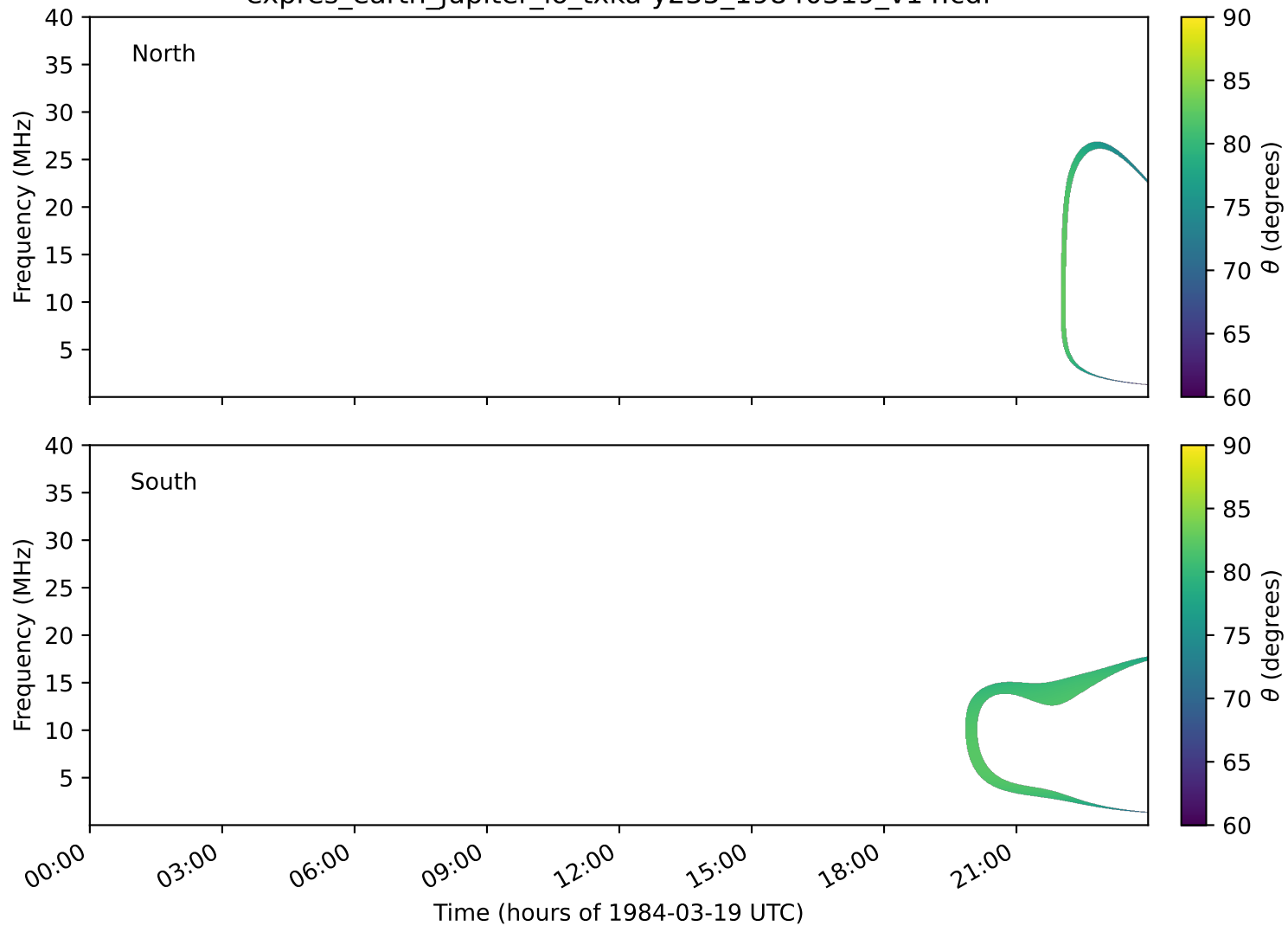
expres_earth_jupiter_io_txka-y235_19840319_v14.cdf
