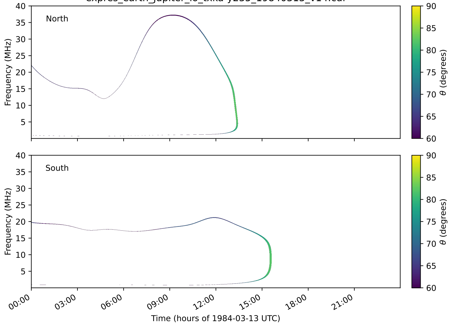
expres_earth_jupiter_io_txka-y235_19840313_v14.cdf
